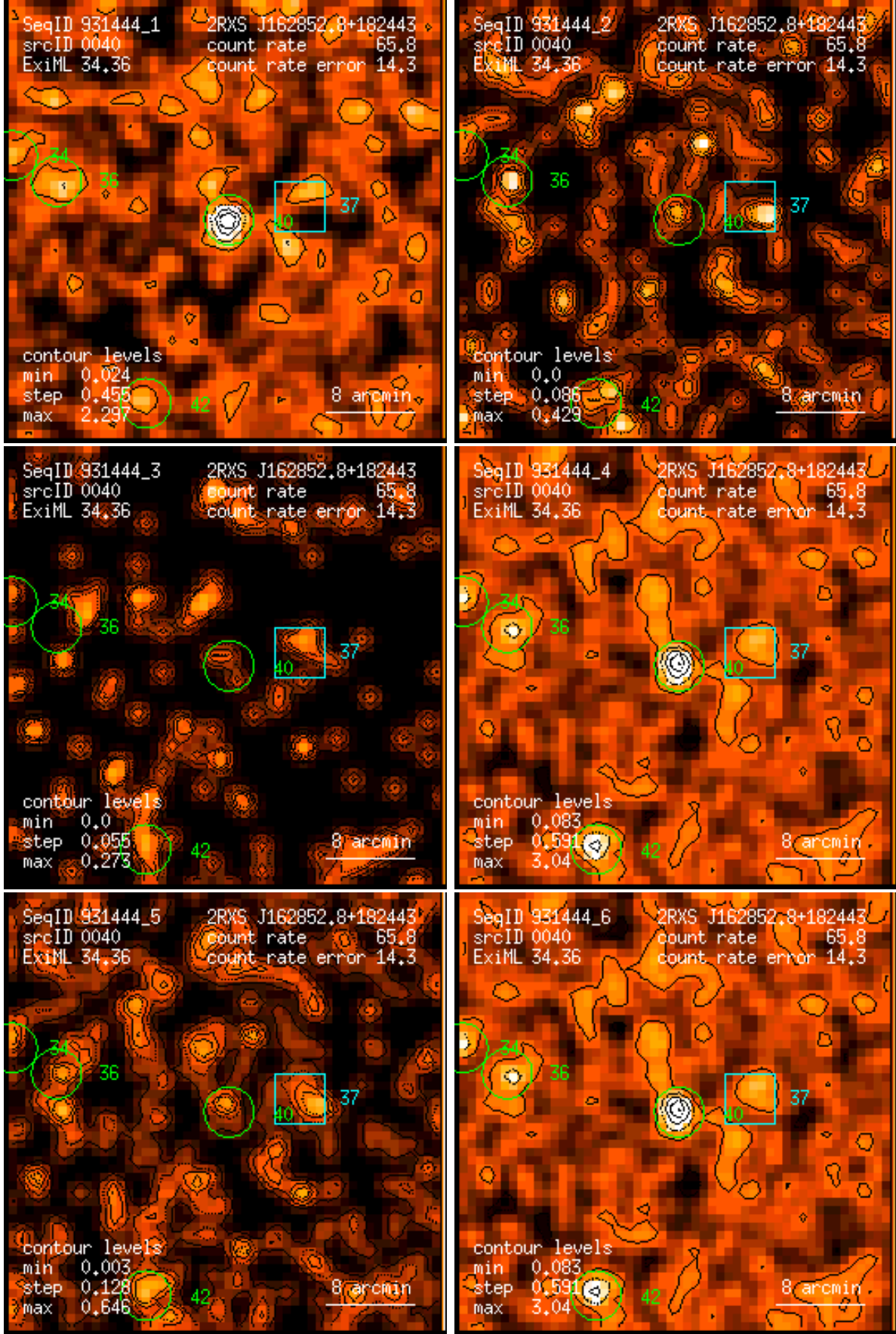
Figure 40: RASS 931444: detection 0040: band rate images, Gaussian filter: (1) PSPC channels 11 – 41, (2) 52 – 90, (3) 91 – 201, (4) 11 – 235, (5) 52 – 201, (6) 11 – 201. Broad band rates in counts/ks. Band rate contour levels in counts/ks/arcmin 2 .
