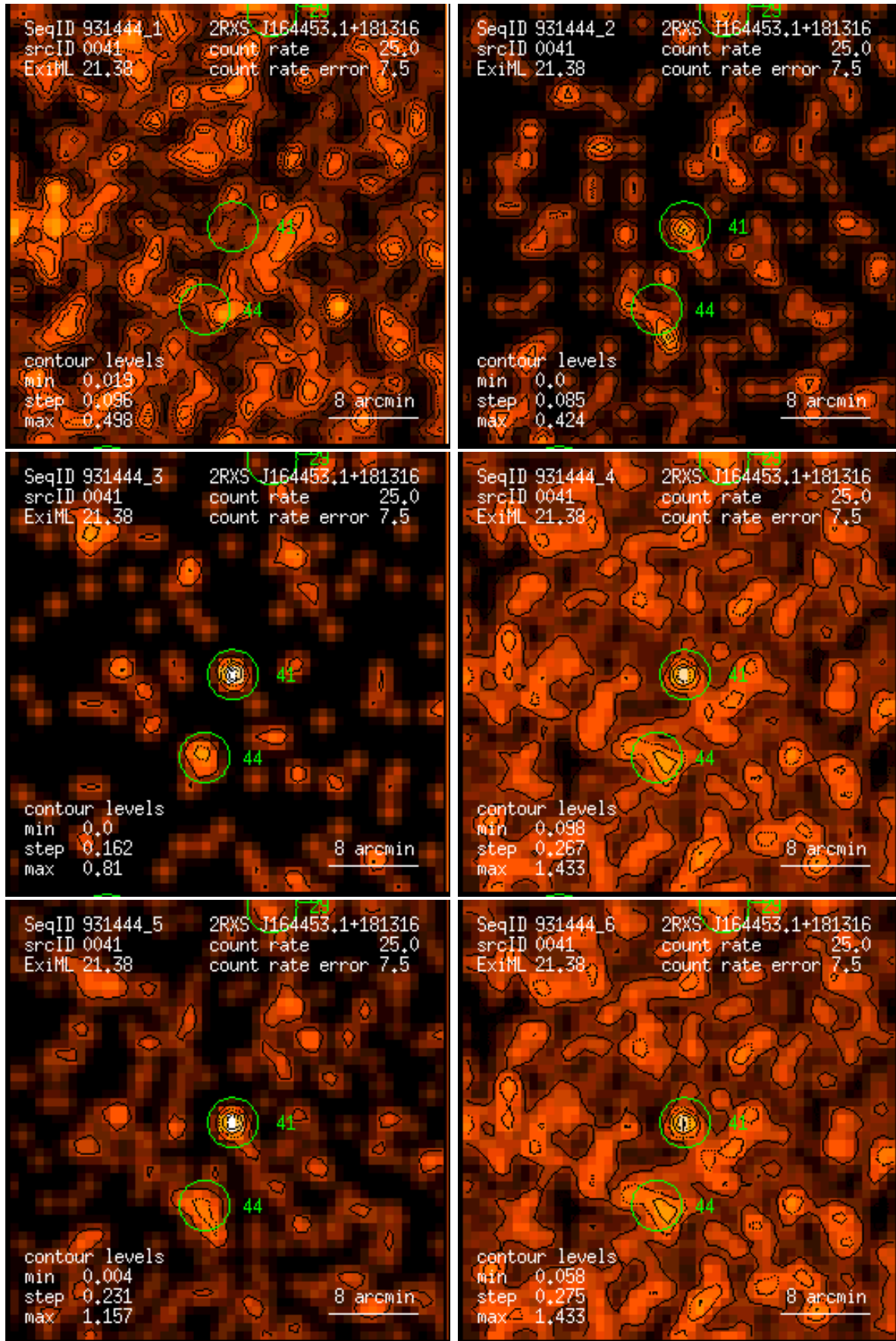
Figure 41: RASS 931444: detection 0041: band rate images, Gaussian filter: (1) PSPC channels 11 – 41, (2) 52 – 90, (3) 91 – 201, (4) 11 – 235, (5) 52 – 201, (6) 11 – 201. Broad band rates in counts/ks. Band rate contour levels in counts/ks/arcmin 2 .
