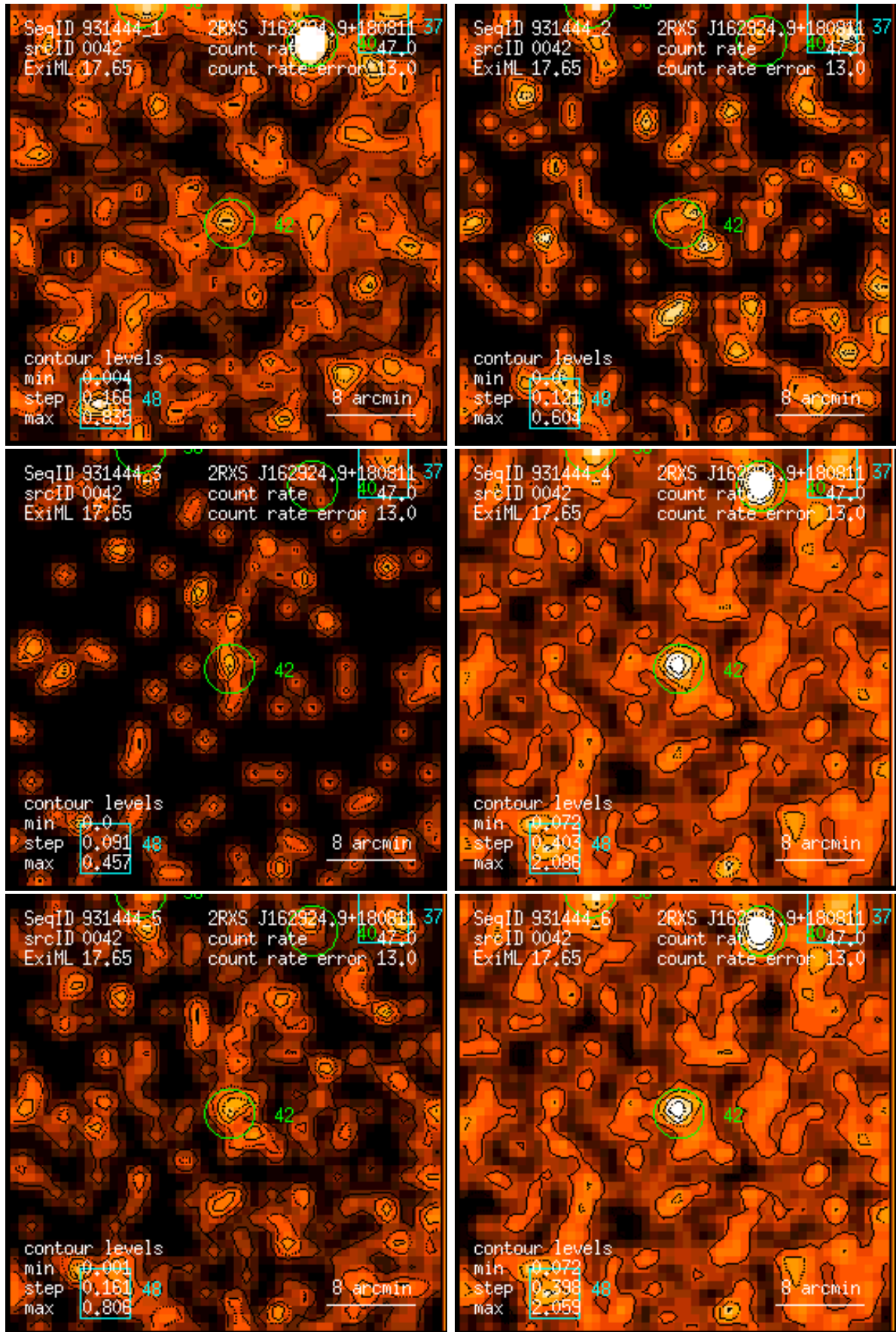
Figure 42: RASS 931444: detection 0042: band rate images, Gaussian filter: (1) PSPC channels 11 – 41, (2) 52 – 90, (3) 91 – 201, (4) 11 – 235, (5) 52 – 201, (6) 11 – 201. Broad band rates in counts/ks. Band rate contour levels in counts/ks/arcmin 2 .
