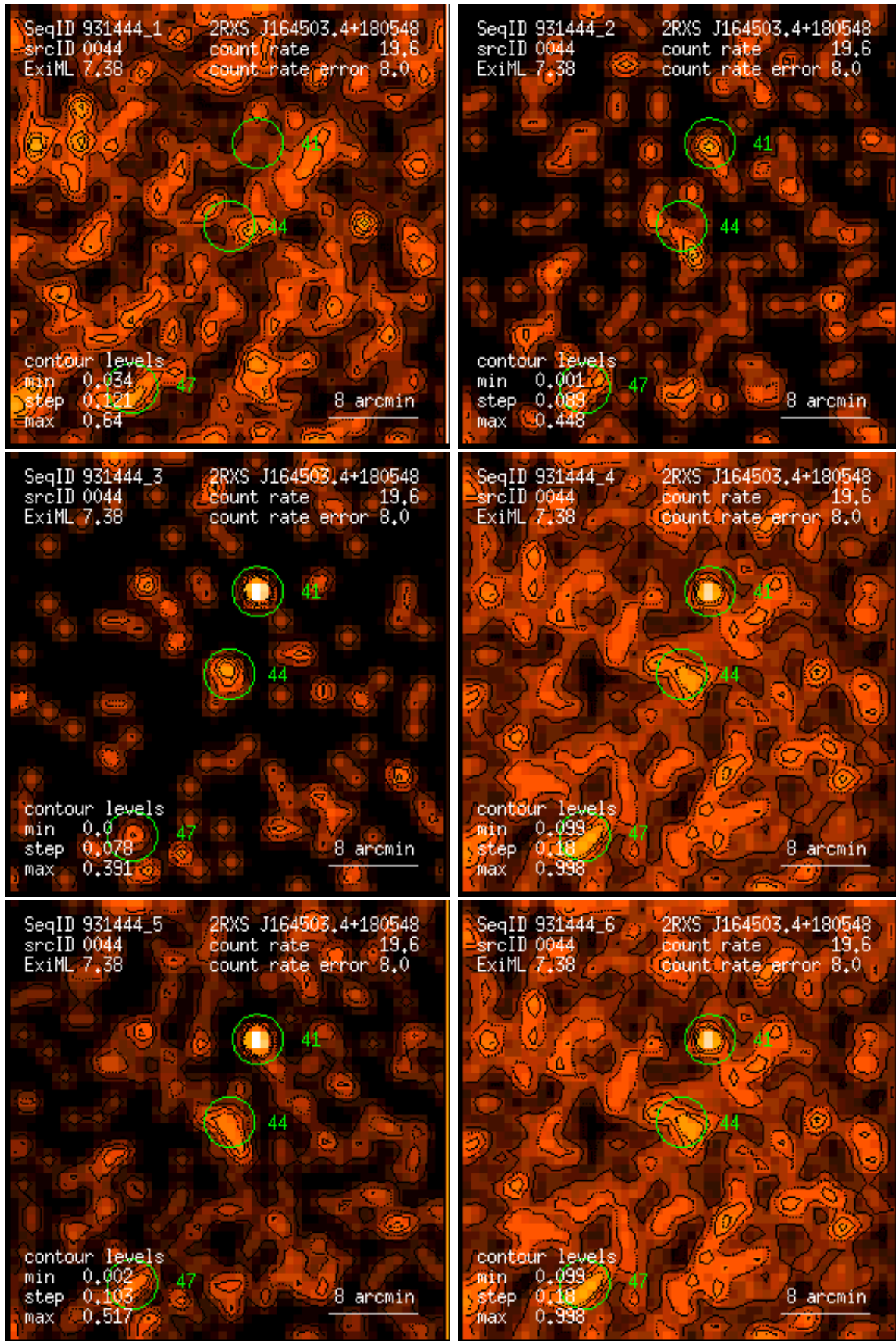
Figure 44: RASS 931444: detection 0044: band rate images, Gaussian filter: (1) PSPC channels 11 – 41, (2) 52 – 90, (3) 91 – 201, (4) 11 – 235, (5) 52 – 201, (6) 11 – 201. Broad band rates in counts/ks. Band rate contour levels in counts/ks/arcmin 2 .
