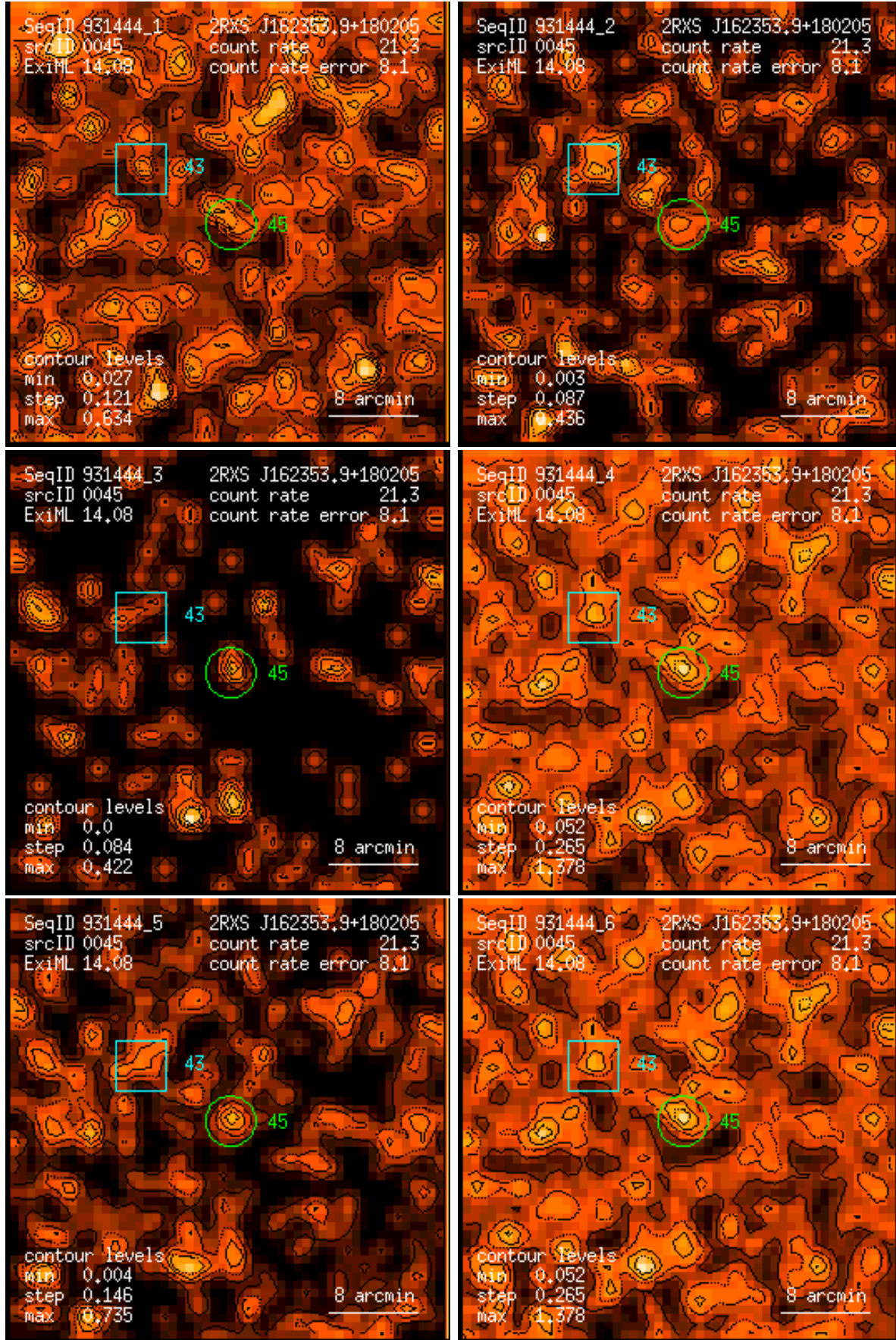
Figure 45: RASS 931444: detection 0045: band rate images, Gaussian filter: (1) PSPC channels 11 – 41, (2) 52 – 90, (3) 91 – 201, (4) 11 – 235, (5) 52 – 201, (6) 11 – 201. Broad band rates in counts/ks. Band rate contour levels in counts/ks/arcmin 2 .
