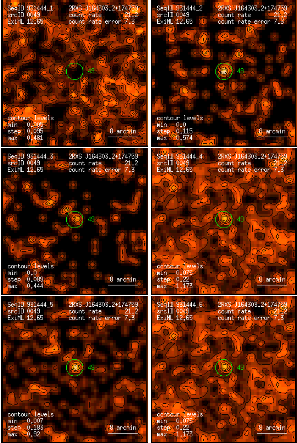
Figure 49: RASS 931444: detection 0049: band rate images, Gaussian filter: (1) PSPC channels 11 – 41, (2) 52 – 90, (3) 91 – 201, (4) 11 – 235, (5) 52 – 201, (6) 11 – 201. Broad band rates in counts/ks. Band rate contour levels in counts/ks/arcmin 2 .
