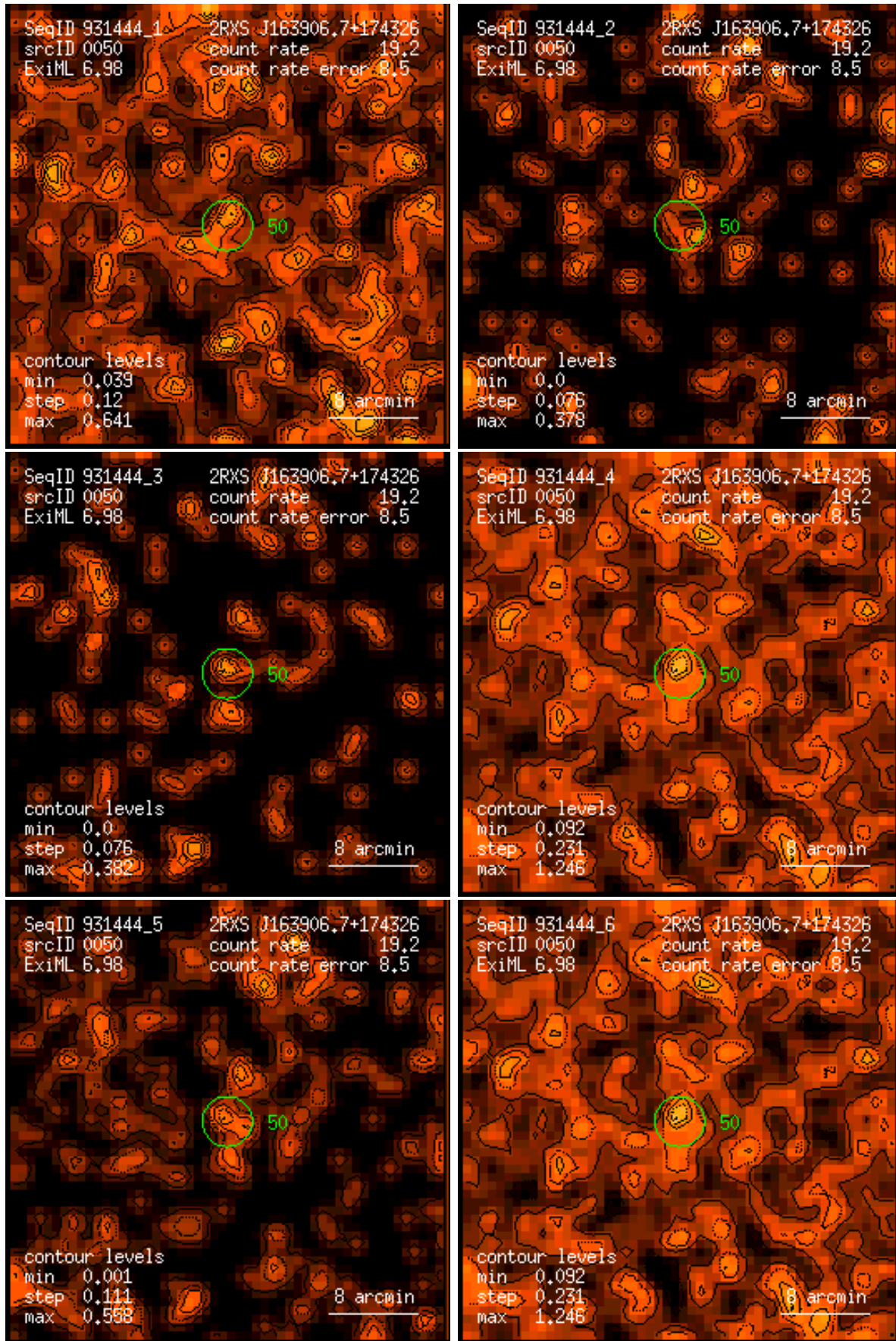
Figure 50: RASS 931444: detection 0050: band rate images, Gaussian filter: (1) PSPC channels 11 – 41, (2) 52 – 90, (3) 91 – 201, (4) 11 – 235, (5) 52 – 201, (6) 11 – 201. Broad band rates in counts/ks. Band rate contour levels in counts/ks/arcmin 2 .
