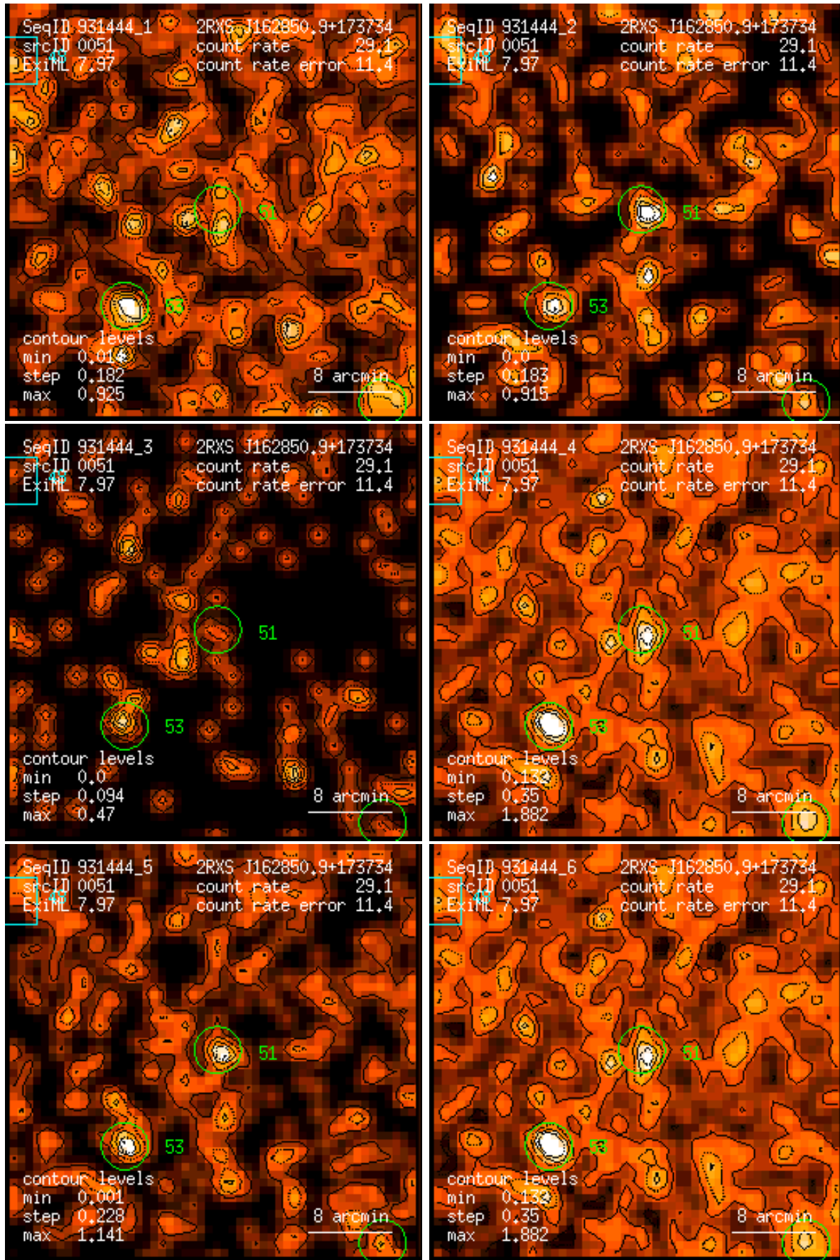
Figure 51: RASS 931444: detection 0051: band rate images, Gaussian filter: (1) PSPC channels 11 – 41, (2) 52 – 90, (3) 91 – 201, (4) 11 – 235, (5) 52 – 201, (6) 11 – 201. Broad band rates in counts/ks. Band rate contour levels in counts/ks/arcmin 2 .
