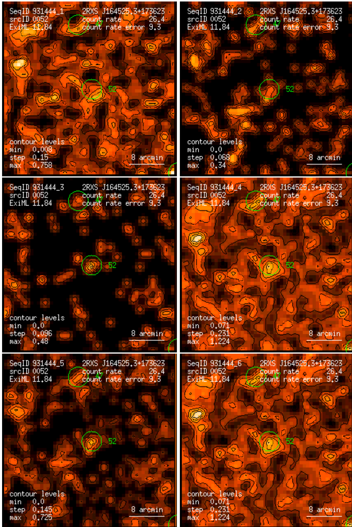
Figure 52: RASS 931444: detection 0052: band rate images, Gaussian filter: (1) PSPC channels 11 – 41, (2) 52 – 90, (3) 91 – 201, (4) 11 – 235, (5) 52 – 201, (6) 11 – 201. Broad band rates in counts/ks. Band rate contour levels in counts/ks/arcmin 2 .
