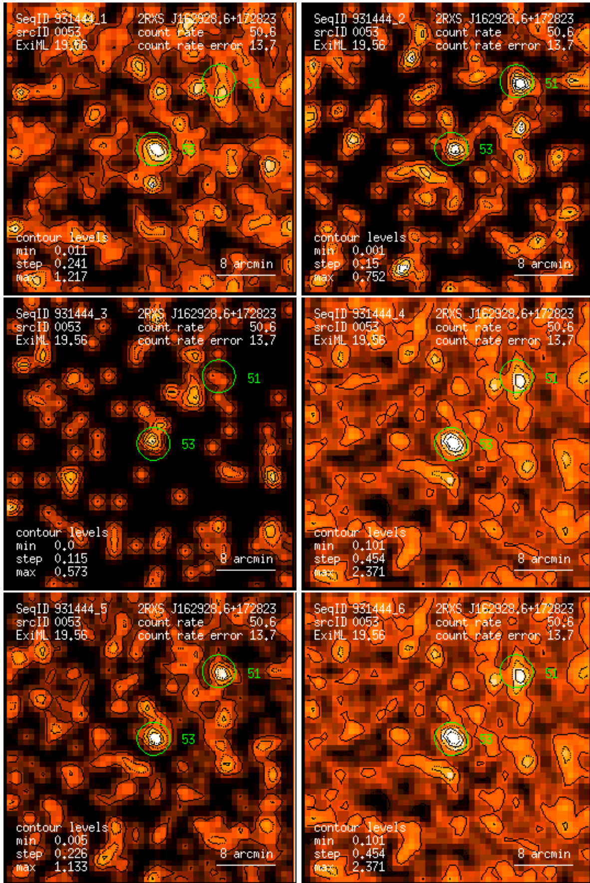
Figure 53: RASS 931444: detection 0053: band rate images, Gaussian filter: (1) PSPC channels 11 – 41, (2) 52 – 90, (3) 91 – 201, (4) 11 – 235, (5) 52 – 201, (6) 11 – 201. Broad band rates in counts/ks. Band rate contour levels in counts/ks/arcmin 2 .
