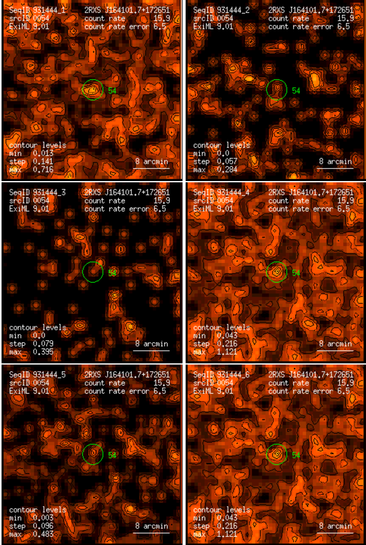
Figure 54: RASS 931444: detection 0054: band rate images, Gaussian filter: (1) PSPC channels 11 – 41, (2) 52 – 90, (3) 91 – 201, (4) 11 – 235, (5) 52 – 201, (6) 11 – 201. Broad band rates in counts/ks. Band rate contour levels in counts/ks/arcmin 2 .
