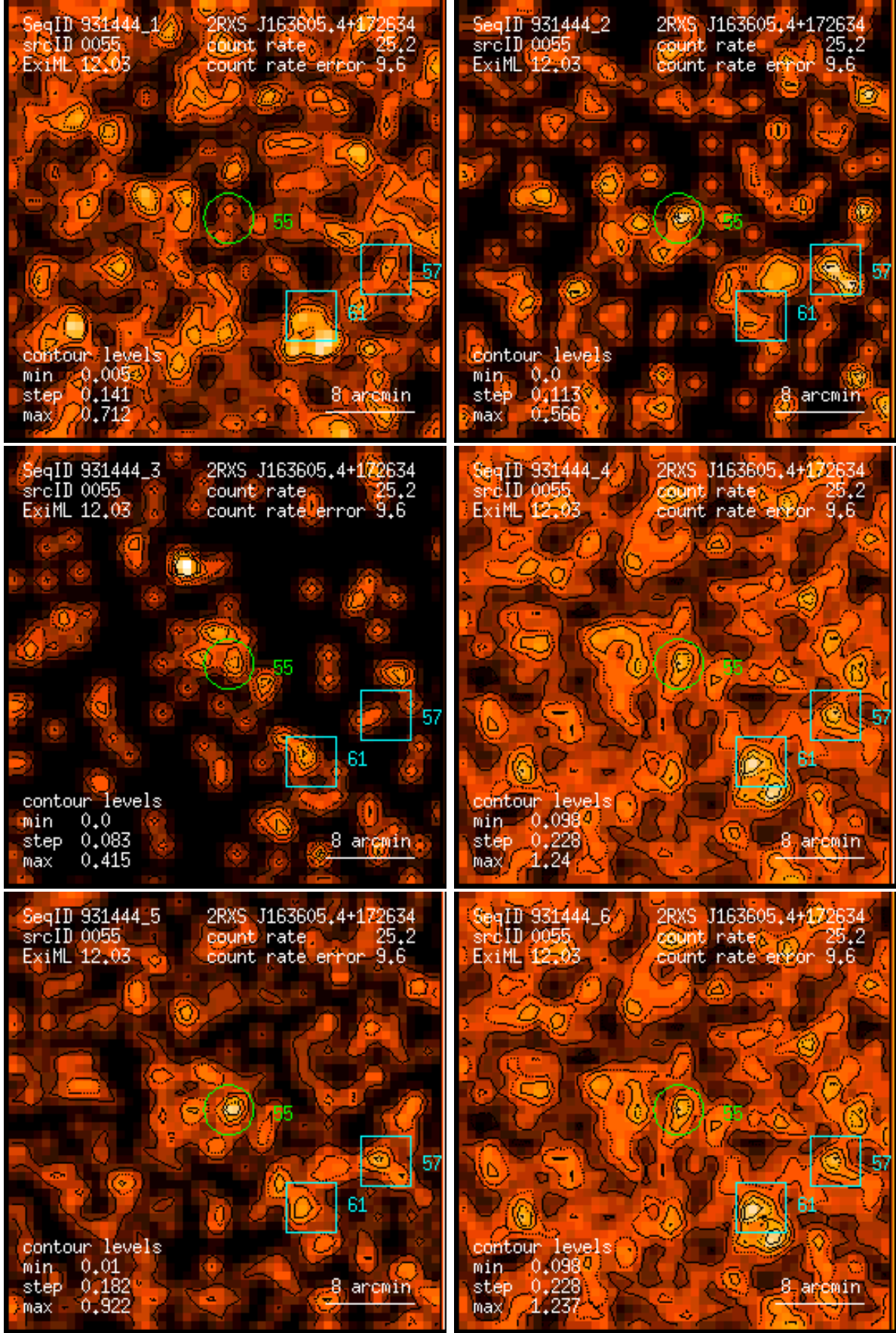
Figure 55: RASS 931444: detection 0055: band rate images, Gaussian filter: (1) PSPC channels 11 – 41, (2) 52 – 90, (3) 91 – 201, (4) 11 – 235, (5) 52 – 201, (6) 11 – 201. Broad band rates in counts/ks. Band rate contour levels in counts/ks/arcmin 2 .
