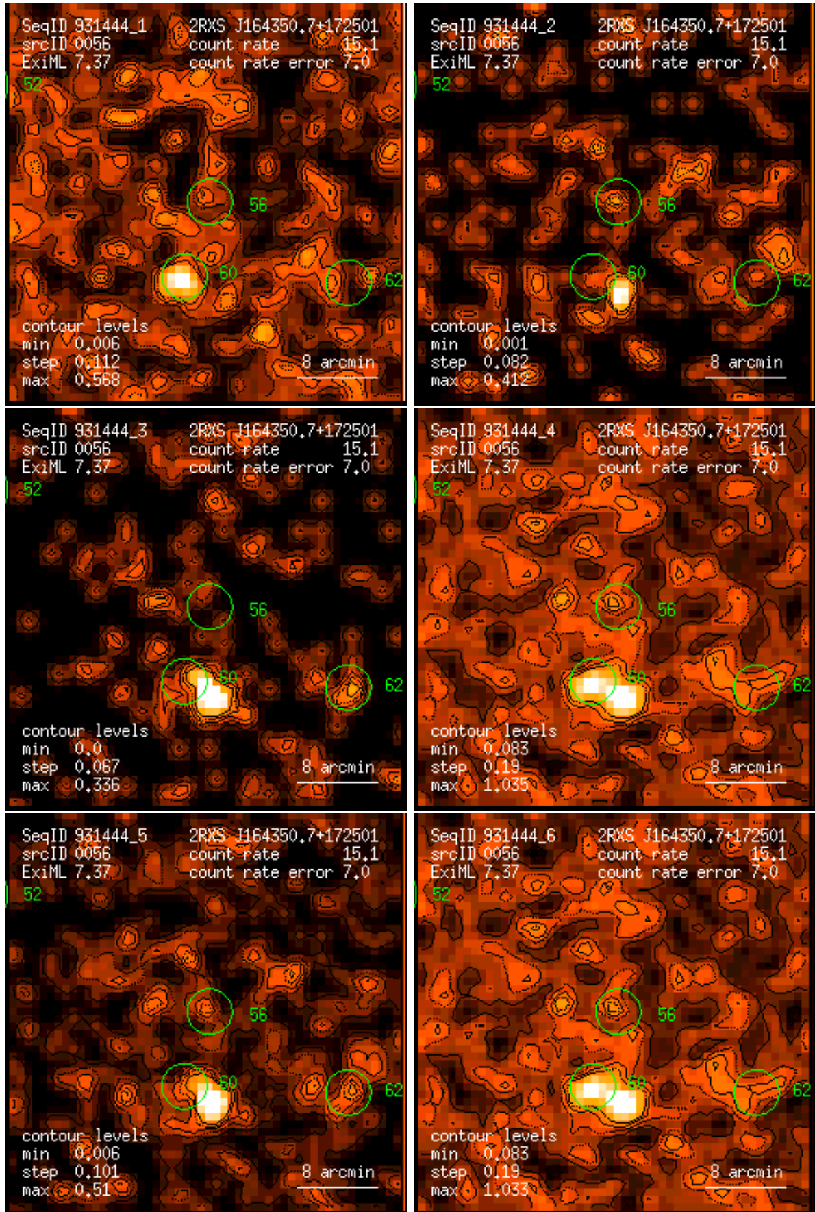
Figure 56: RASS 931444: detection 0056: band rate images, Gaussian filter: (1) PSPC channels 11 – 41, (2) 52 – 90, (3) 91 – 201, (4) 11 – 235, (5) 52 – 201, (6) 11 – 201. Broad band rates in counts/ks. Band rate contour levels in counts/ks/arcmin 2 .
