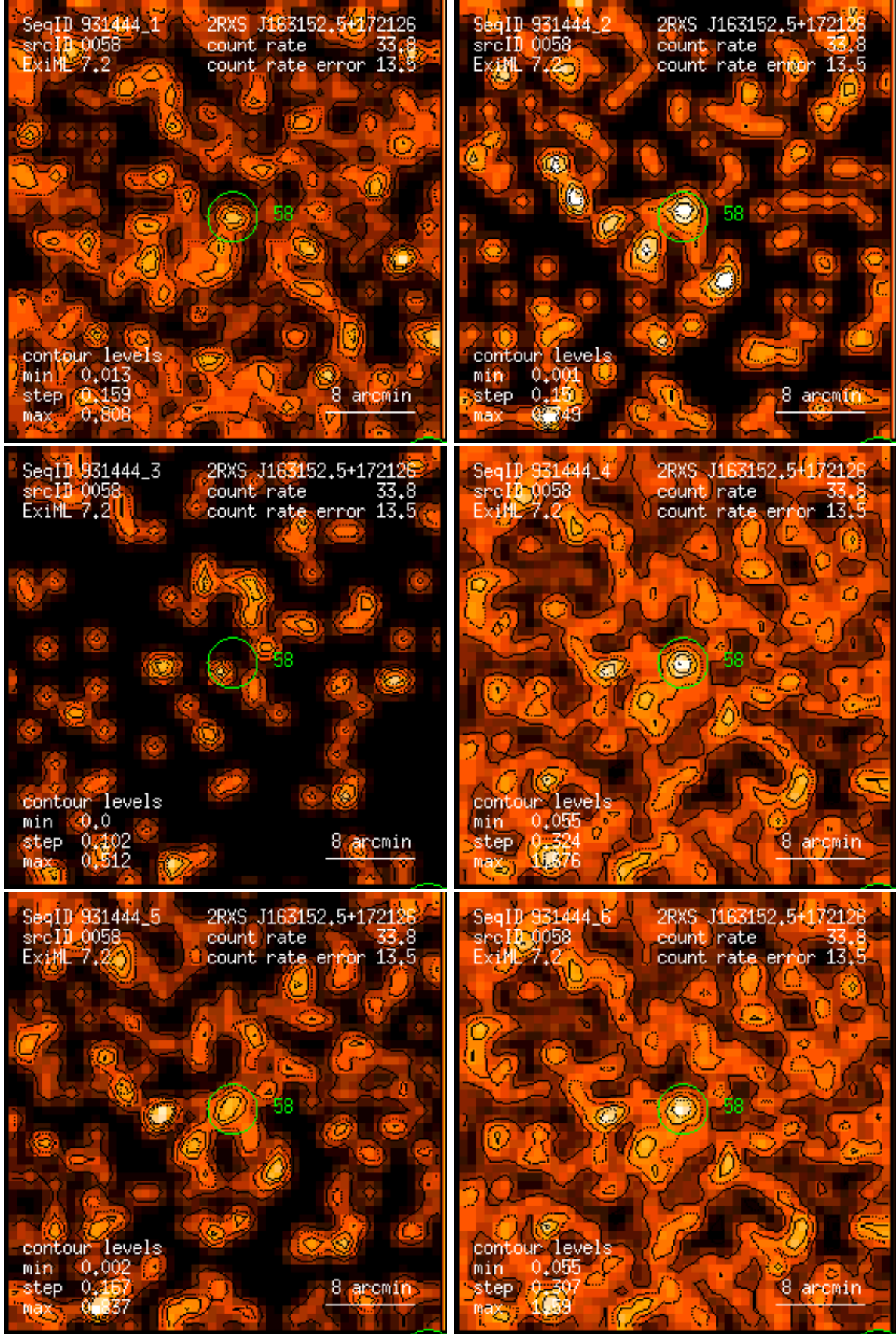
Figure 58: RASS 931444: detection 0058: band rate images, Gaussian filter: (1) PSPC channels 11 – 41, (2) 52 – 90, (3) 91 – 201, (4) 11 – 235, (5) 52 – 201, (6) 11 – 201. Broad band rates in counts/ks. Band rate contour levels in counts/ks/arcmin 2 .
