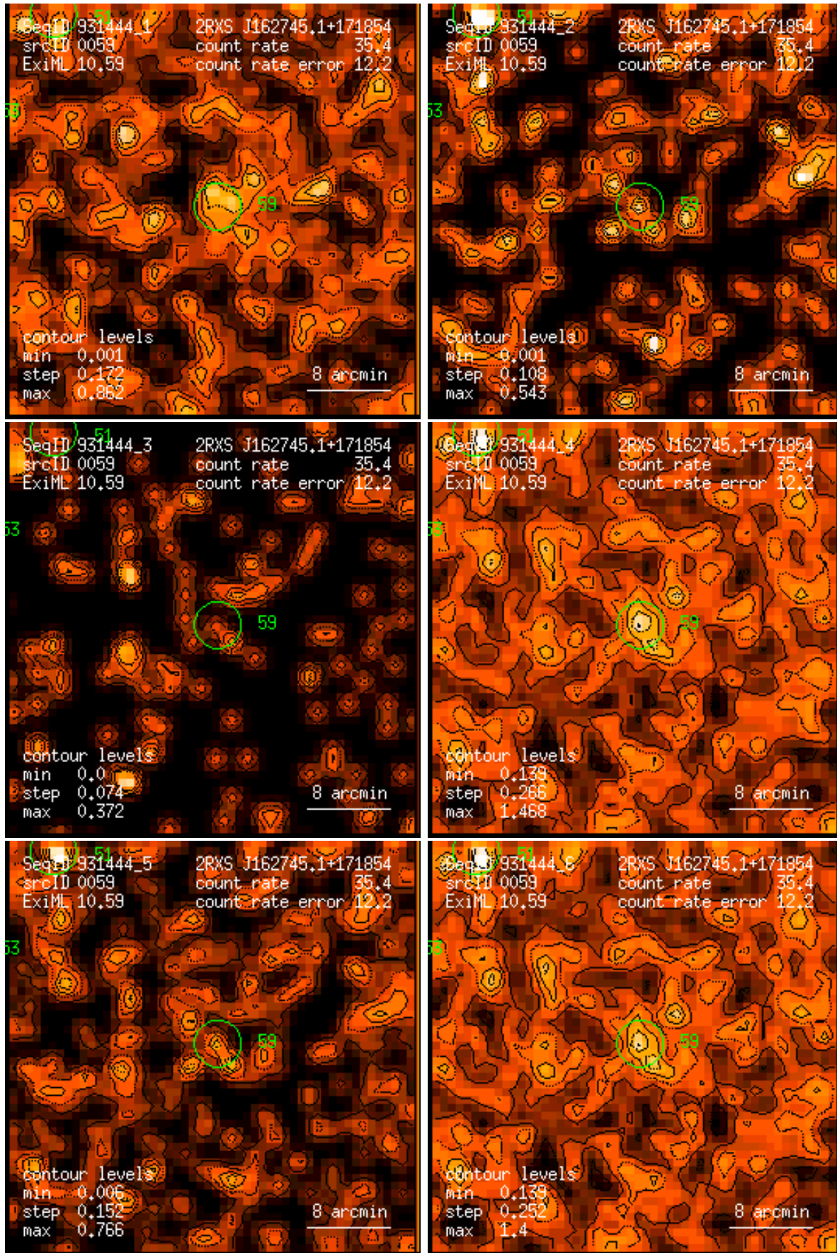
Figure 59: RASS 931444: detection 0059: band rate images, Gaussian filter: (1) PSPC channels 11 – 41, (2) 52 – 90, (3) 91 – 201, (4) 11 – 235, (5) 52 – 201, (6) 11 – 201. Broad band rates in counts/ks. Band rate contour levels in counts/ks/arcmin 2 .
