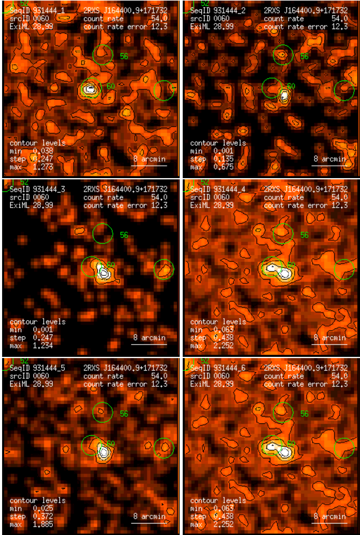
Figure 60: RASS 931444: detection 0060: band rate images, Gaussian filter: (1) PSPC channels 11 – 41, (2) 52 – 90, (3) 91 – 201, (4) 11 – 235, (5) 52 – 201, (6) 11 – 201. Broad band rates in counts/ks. Band rate contour levels in counts/ks/arcmin 2 .
