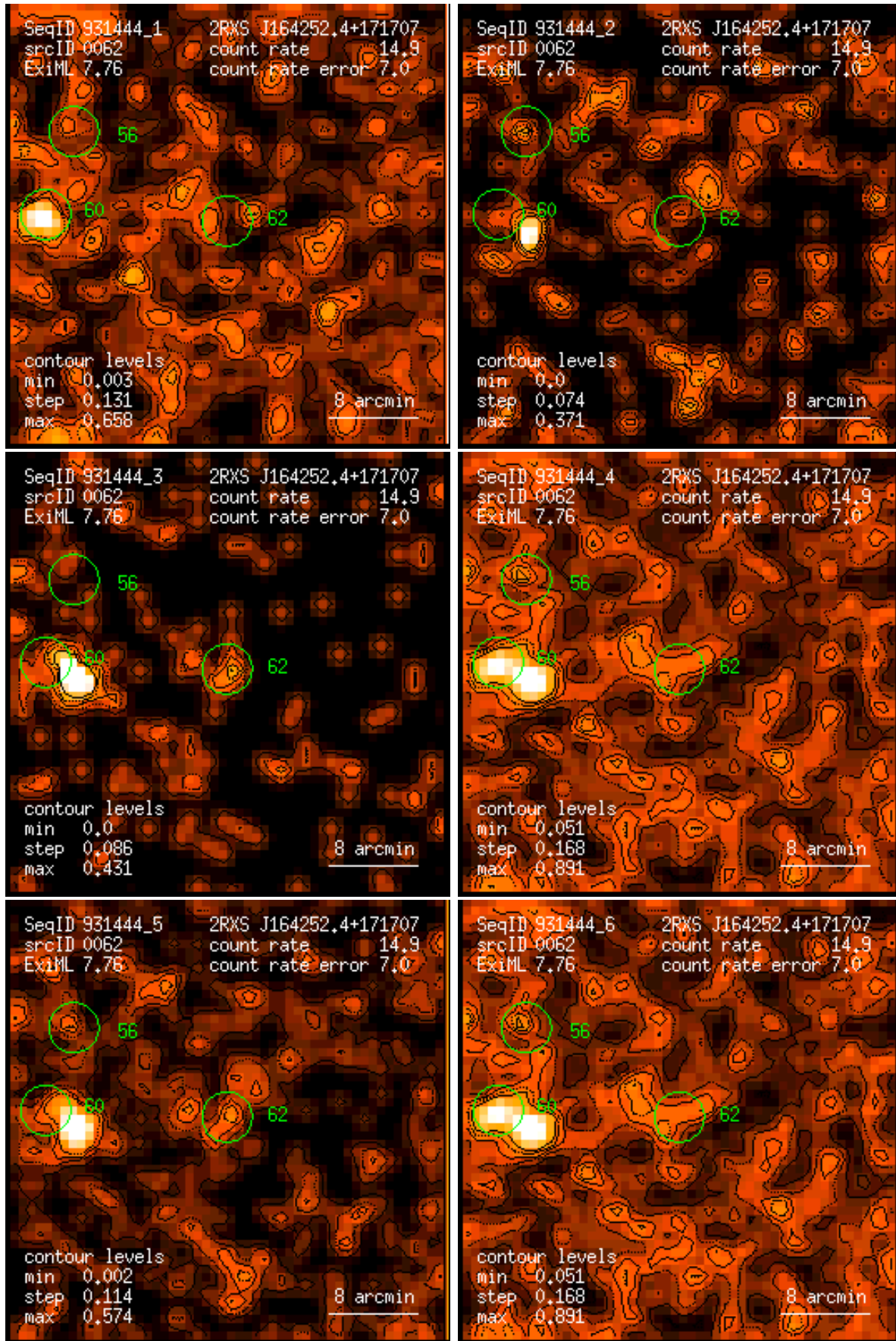
Figure 62: RASS 931444: detection 0062: band rate images, Gaussian filter: (1) PSPC channels 11 – 41, (2) 52 – 90, (3) 91 – 201, (4) 11 – 235, (5) 52 – 201, (6) 11 – 201. Broad band rates in counts/ks. Band rate contour levels in counts/ks/arcmin 2 .
