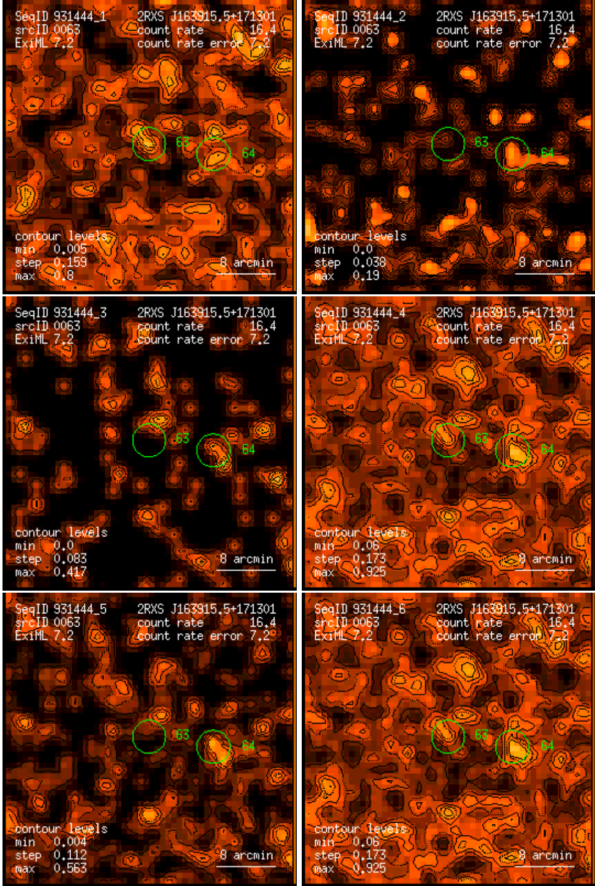
Figure 63: RASS 931444: detection 0063: band rate images, Gaussian filter: (1) PSPC channels 11 – 41, (2) 52 – 90, (3) 91 – 201, (4) 11 – 235, (5) 52 – 201, (6) 11 – 201. Broad band rates in counts/ks. Band rate contour levels in counts/ks/arcmin 2 .
