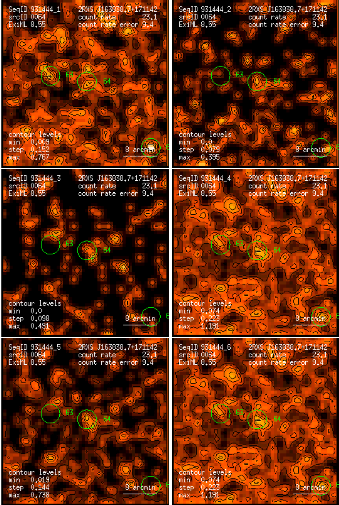
Figure 64: RASS 931444: detection 0064: band rate images, Gaussian filter: (1) PSPC channels 11 – 41, (2) 52 – 90, (3) 91 – 201, (4) 11 – 235, (5) 52 – 201, (6) 11 – 201. Broad band rates in counts/ks. Band rate contour levels in counts/ks/arcmin 2 .
