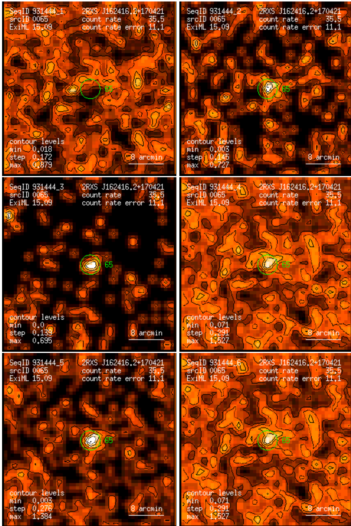
Figure 65: RASS 931444: detection 0065: band rate images, Gaussian filter: (1) PSPC channels 11 – 41, (2) 52 – 90, (3) 91 – 201, (4) 11 – 235, (5) 52 – 201, (6) 11 – 201. Broad band rates in counts/ks. Band rate contour levels in counts/ks/arcmin 2 .
