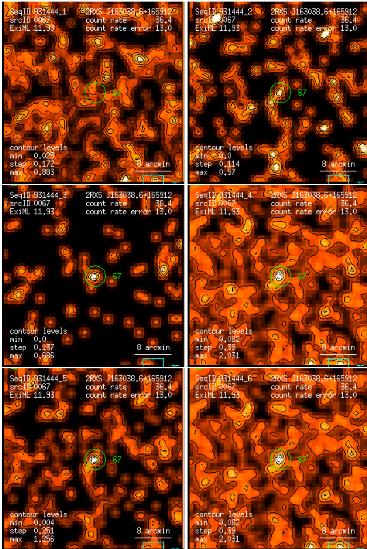
Figure 67: RASS 931444: detection 0067: band rate images, Gaussian filter: (1) PSPC channels 11 – 41, (2) 52 – 90, (3) 91 – 201, (4) 11 – 235, (5) 52 – 201, (6) 11 – 201. Broad band rates in counts/ks. Band rate contour levels in counts/ks/arcmin 2 .
