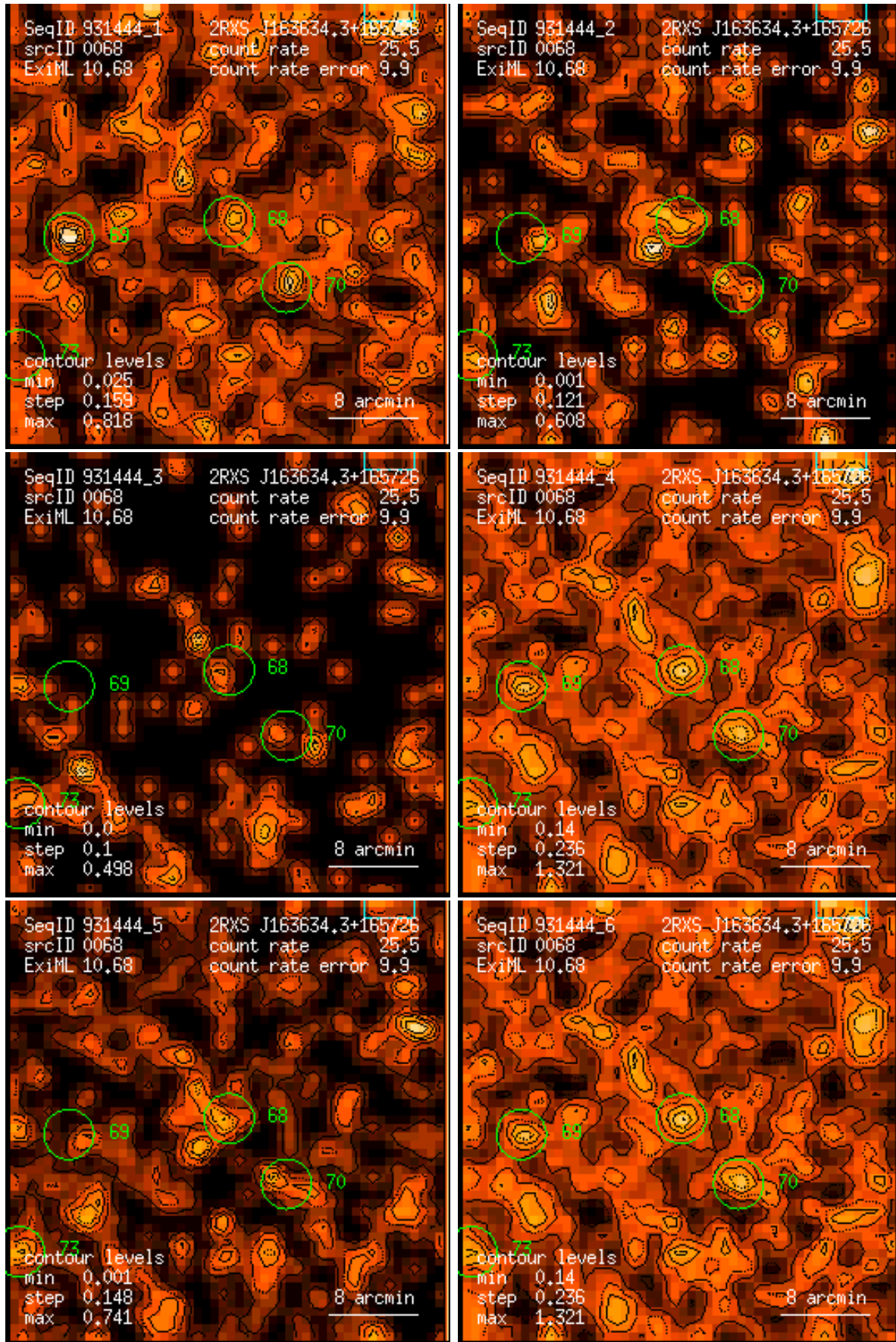
Figure 68: RASS 931444: detection 0068: band rate images, Gaussian filter: (1) PSPC channels 11 – 41, (2) 52 – 90, (3) 91 – 201, (4) 11 – 235, (5) 52 – 201, (6) 11 – 201. Broad band rates in counts/ks. Band rate contour levels in counts/ks/arcmin 2 .
