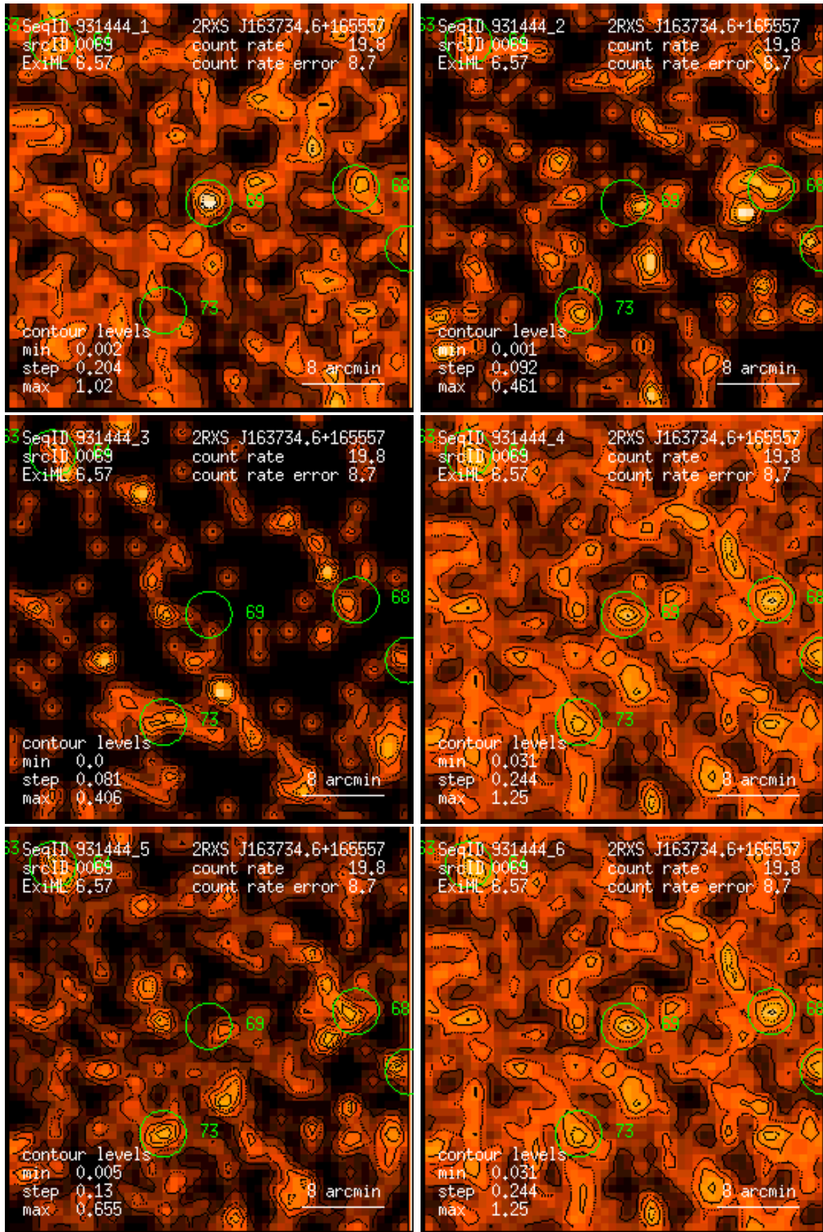
Figure 69: RASS 931444: detection 0069: band rate images, Gaussian filter: (1) PSPC channels 11 – 41, (2) 52 – 90, (3) 91 – 201, (4) 11 – 235, (5) 52 – 201, (6) 11 – 201. Broad band rates in counts/ks. Band rate contour levels in counts/ks/arcmin 2 .
