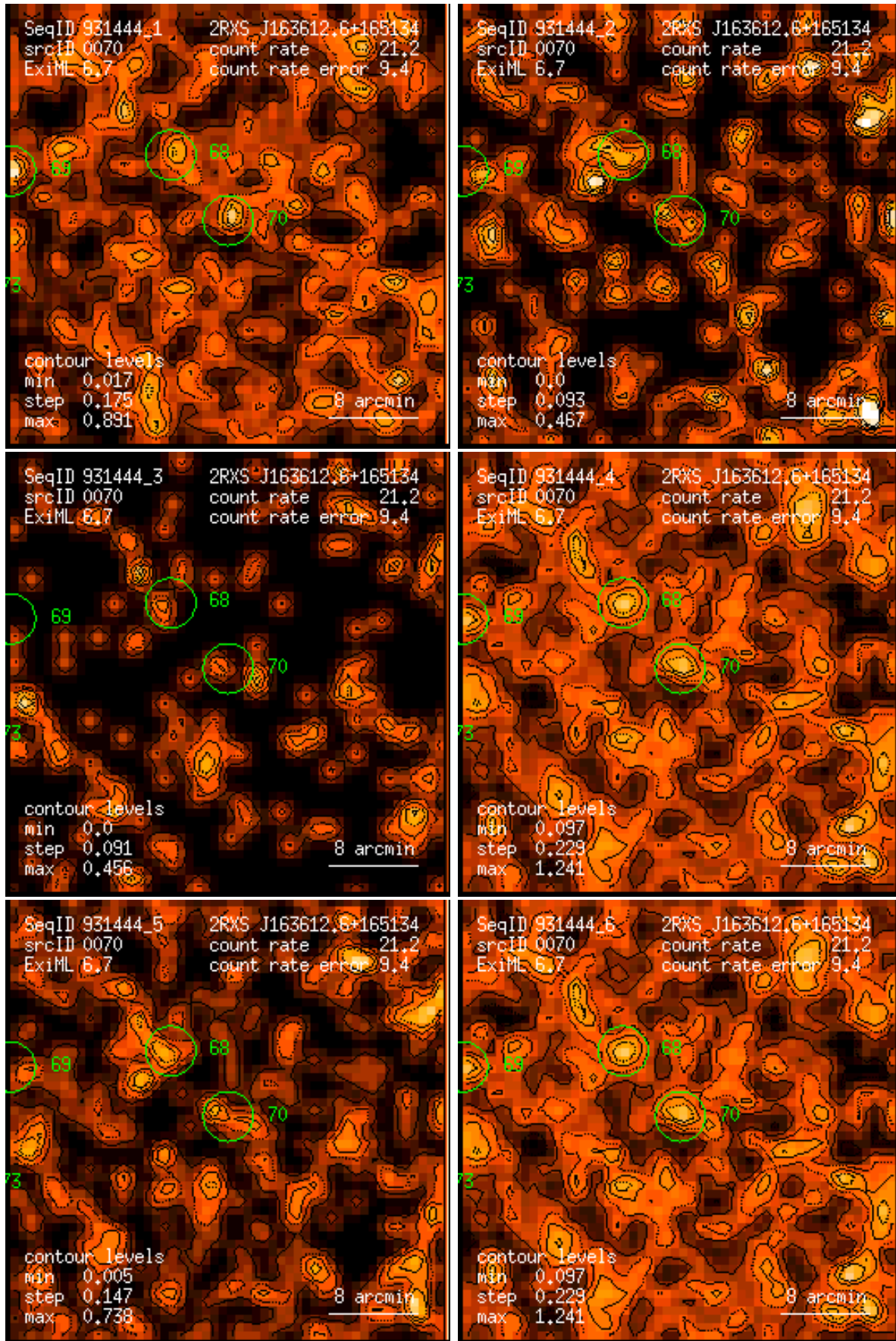
Figure 70: RASS 931444: detection 0070: band rate images, Gaussian filter: (1) PSPC channels 11 – 41, (2) 52 – 90, (3) 91 – 201, (4) 11 – 235, (5) 52 – 201, (6) 11 – 201. Broad band rates in counts/ks. Band rate contour levels in counts/ks/arcmin 2 .
