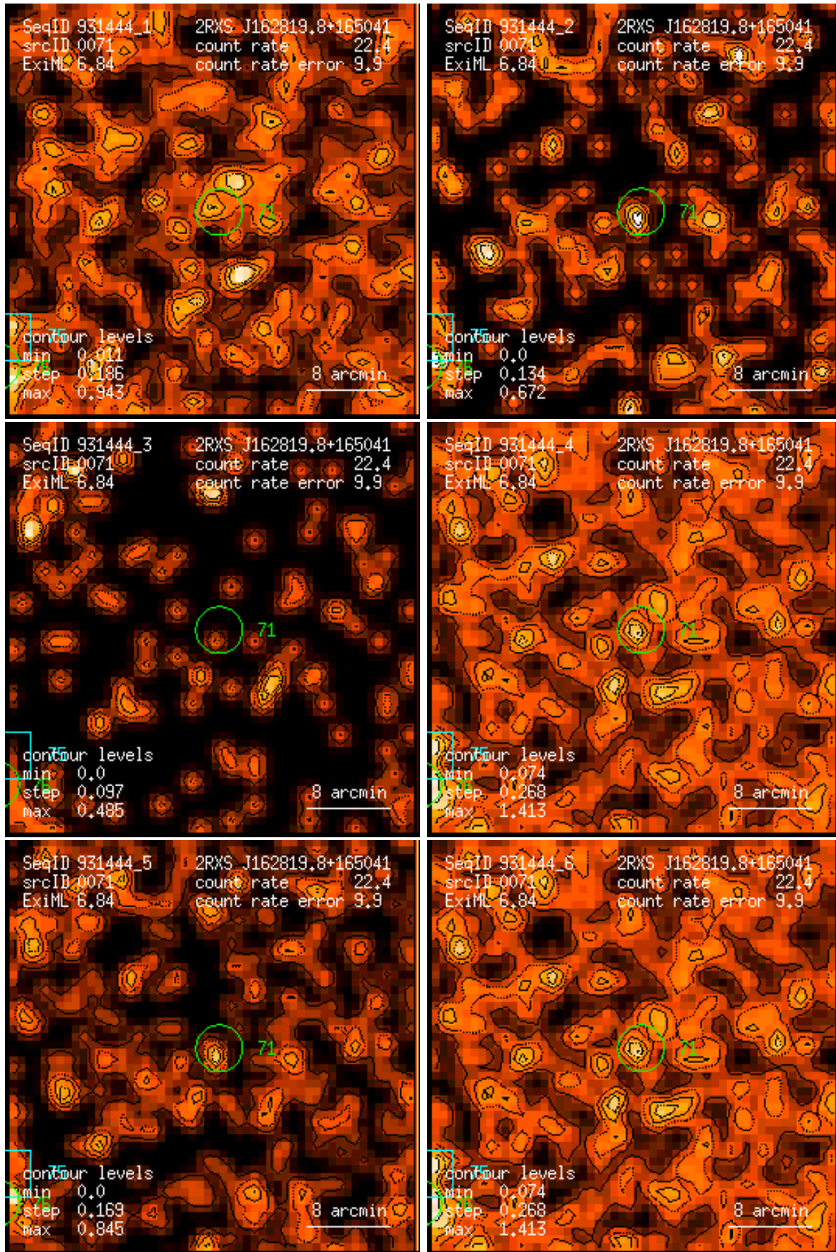
Figure 71: RASS 931444: detection 0071: band rate images, Gaussian filter: (1) PSPC channels 11 – 41, (2) 52 – 90, (3) 91 – 201, (4) 11 – 235, (5) 52 – 201, (6) 11 – 201. Broad band rates in counts/ks. Band rate contour levels in counts/ks/arcmin 2 .
