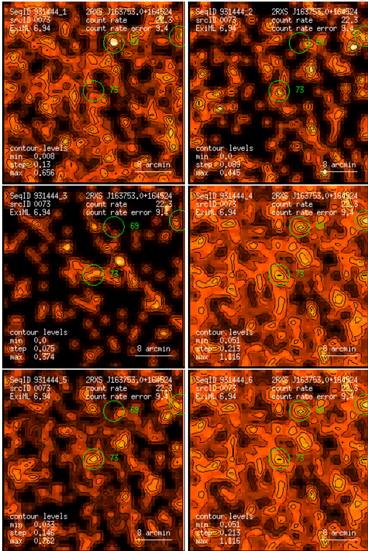
Figure 73: RASS 931444: detection 0073: band rate images, Gaussian filter: (1) PSPC channels 11 – 41, (2) 52 – 90, (3) 91 – 201, (4) 11 – 235, (5) 52 – 201, (6) 11 – 201. Broad band rates in counts/ks. Band rate contour levels in counts/ks/arcmin 2 .
