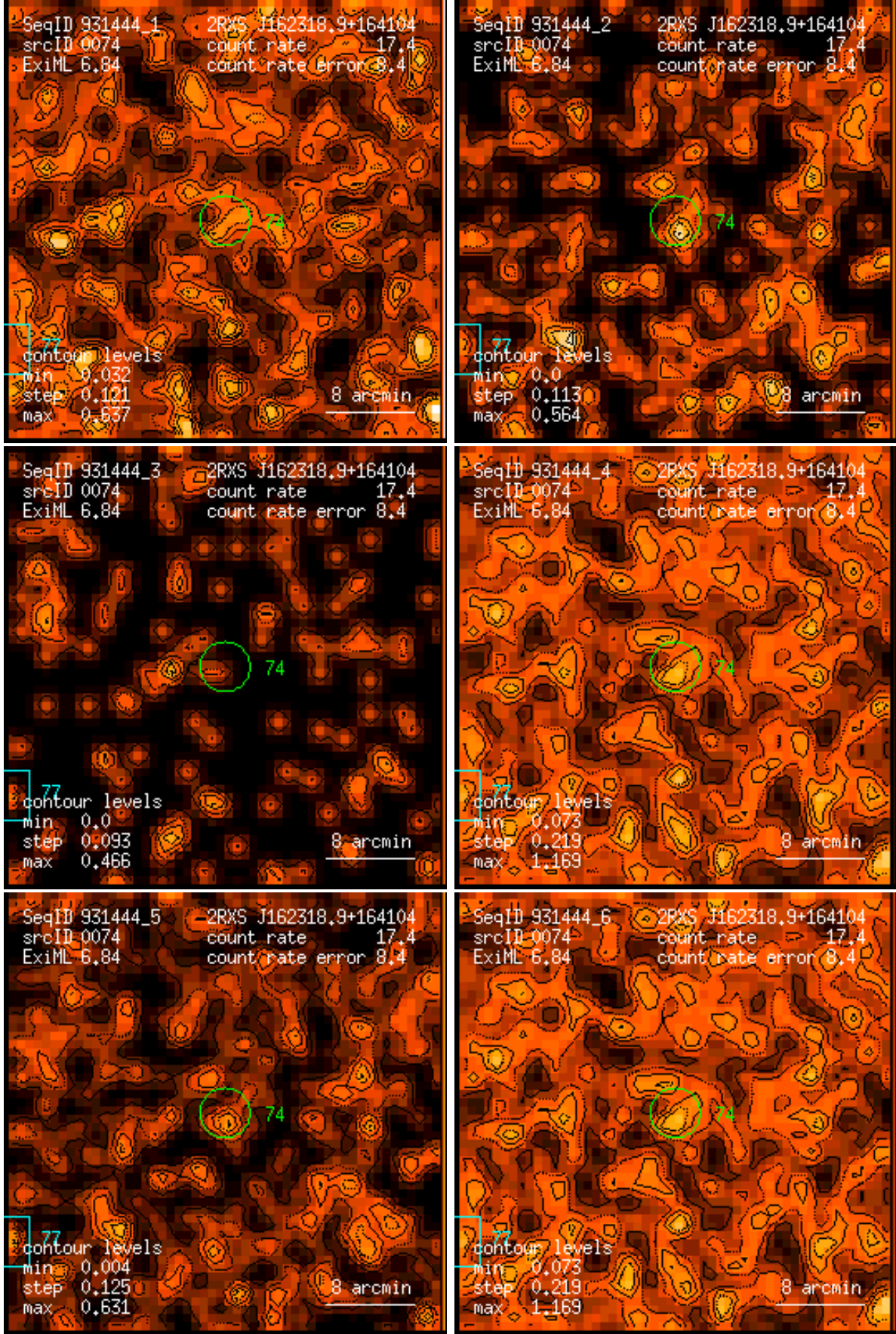
Figure 74: RASS 931444: detection 0074: band rate images, Gaussian filter: (1) PSPC channels 11 – 41, (2) 52 – 90, (3) 91 – 201, (4) 11 – 235, (5) 52 – 201, (6) 11 – 201. Broad band rates in counts/ks. Band rate contour levels in counts/ks/arcmin 2 .
