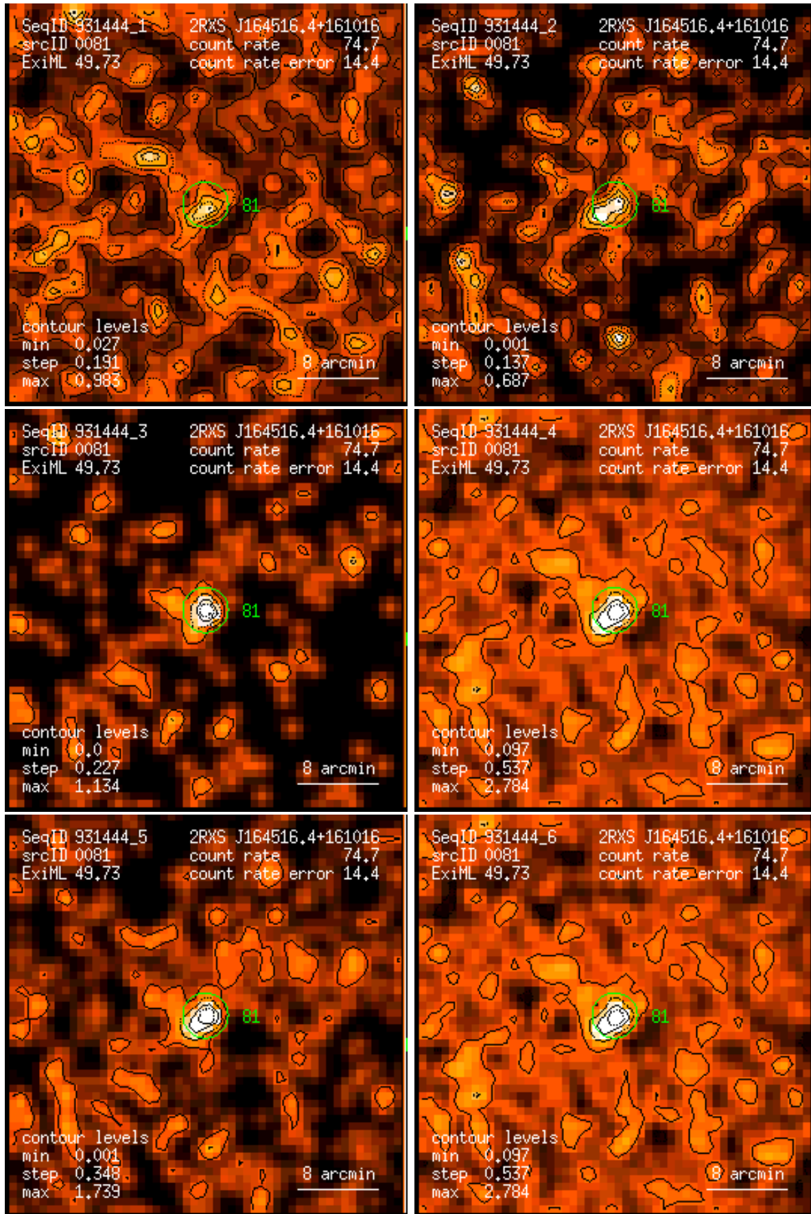
Figure 81: RASS 931444: detection 0081: band rate images, Gaussian filter: (1) PSPC channels 11 – 41, (2) 52 – 90, (3) 91 – 201, (4) 11 – 235, (5) 52 – 201, (6) 11 – 201. Broad band rates in counts/ks. Band rate contour levels in counts/ks/arcmin 2 .
