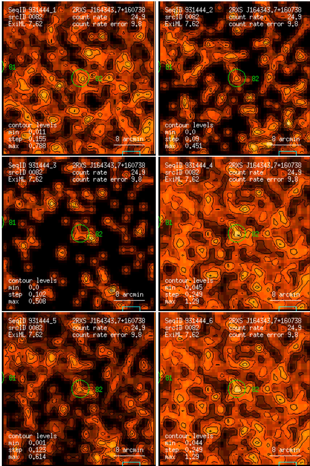
Figure 82: RASS 931444: detection 0082: band rate images, Gaussian filter: (1) PSPC channels 11 – 41, (2) 52 – 90, (3) 91 – 201, (4) 11 – 235, (5) 52 – 201, (6) 11 – 201. Broad band rates in counts/ks. Band rate contour levels in counts/ks/arcmin 2 .
