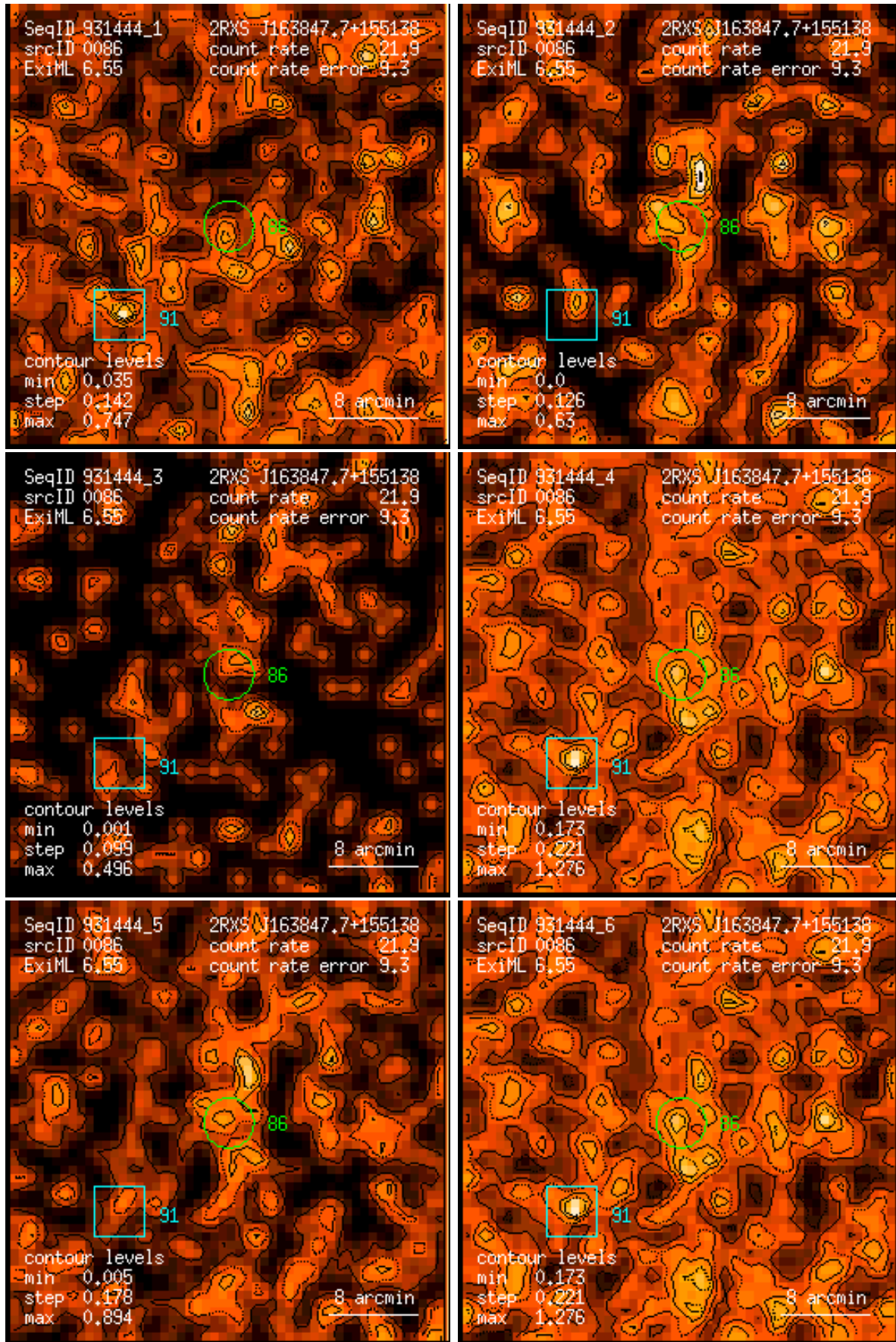
Figure 86: RASS 931444: detection 0086: band rate images, Gaussian filter: (1) PSPC channels 11 – 41, (2) 52 – 90, (3) 91 – 201, (4) 11 – 235, (5) 52 – 201, (6) 11 – 201. Broad band rates in counts/ks. Band rate contour levels in counts/ks/arcmin 2 .
