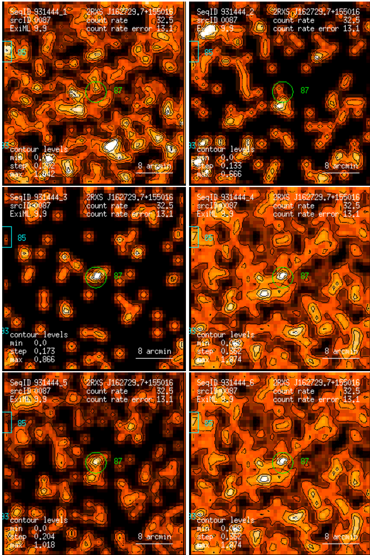
Figure 87: RASS 931444: detection 0087: band rate images, Gaussian filter: (1) PSPC channels 11 – 41, (2) 52 – 90, (3) 91 – 201, (4) 11 – 235, (5) 52 – 201, (6) 11 – 201. Broad band rates in counts/ks. Band rate contour levels in counts/ks/arcmin 2 .
