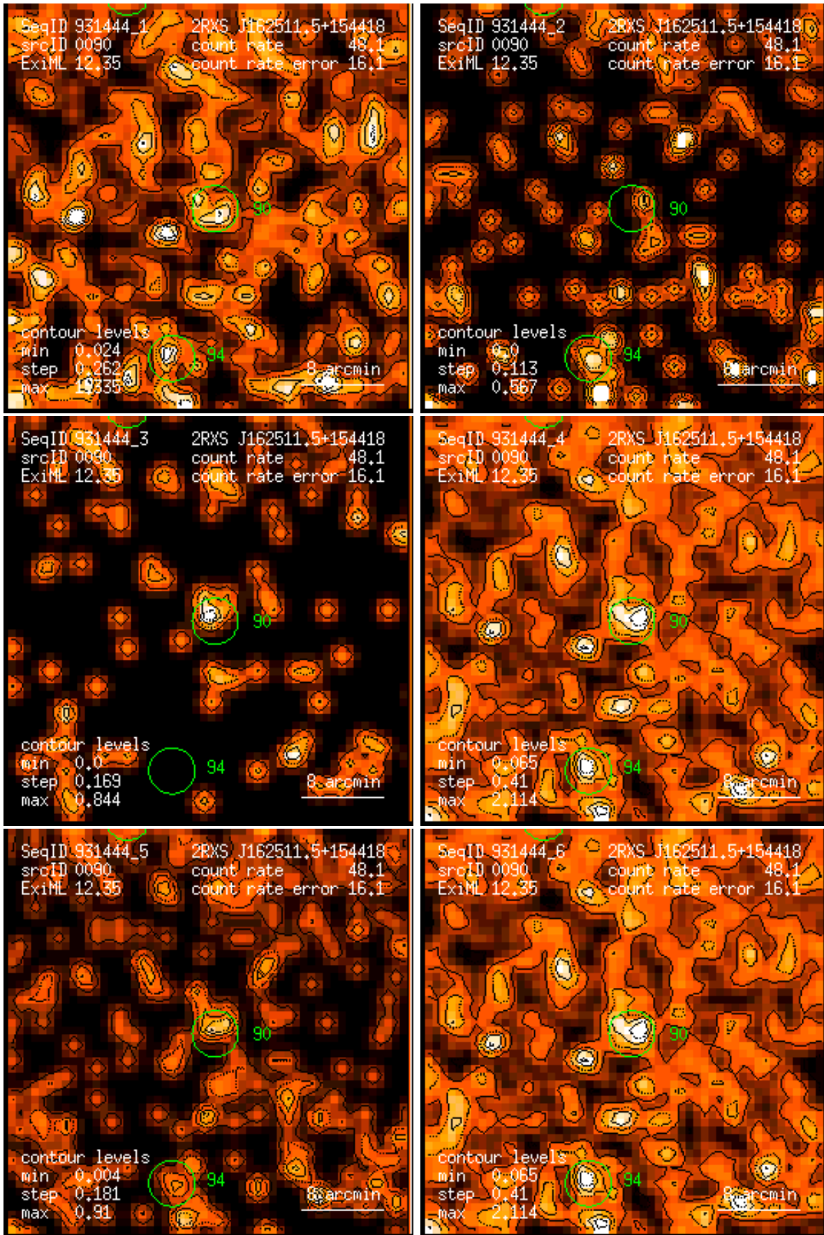
Figure 90: RASS 931444: detection 0090: band rate images, Gaussian filter: (1) PSPC channels 11 – 41, (2) 52 – 90, (3) 91 – 201, (4) 11 – 235, (5) 52 – 201, (6) 11 – 201. Broad band rates in counts/ks. Band rate contour levels in counts/ks/arcmin 2 .
