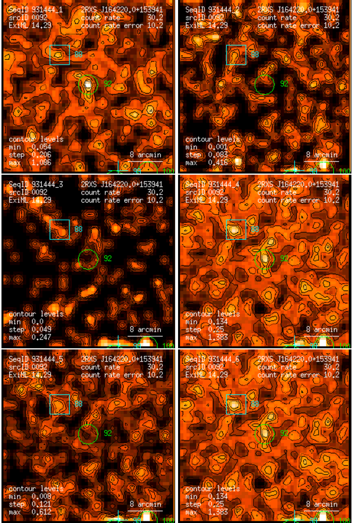
Figure 92: RASS 931444: detection 0092: band rate images, Gaussian filter: (1) PSPC channels 11 – 41, (2) 52 – 90, (3) 91 – 201, (4) 11 – 235, (5) 52 – 201, (6) 11 – 201. Broad band rates in counts/ks. Band rate contour levels in counts/ks/arcmin 2 .
