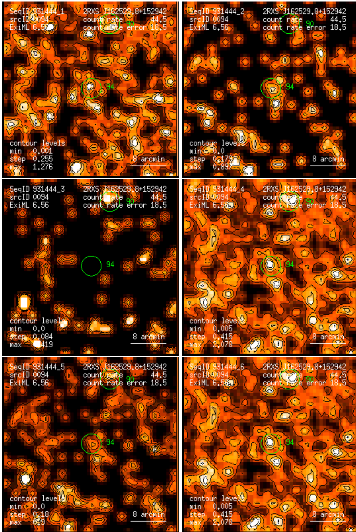
Figure 94: RASS 931444: detection 0094: band rate images, Gaussian filter: (1) PSPC channels 11 – 41, (2) 52 – 90, (3) 91 – 201, (4) 11 – 235, (5) 52 – 201, (6) 11 – 201. Broad band rates in counts/ks. Band rate contour levels in counts/ks/arcmin 2 .
