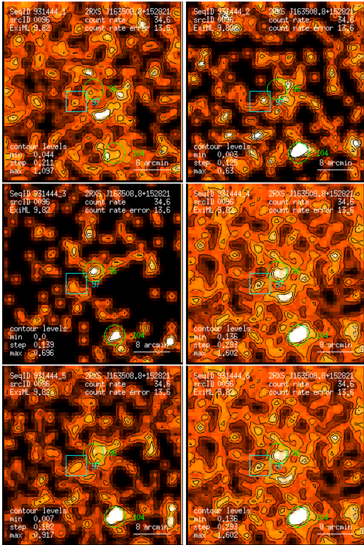
Figure 96: RASS 931444: detection 0096: band rate images, Gaussian filter: (1) PSPC channels 11 – 41, (2) 52 – 90, (3) 91 – 201, (4) 11 – 235, (5) 52 – 201, (6) 11 – 201. Broad band rates in counts/ks. Band rate contour levels in counts/ks/arcmin 2 .
