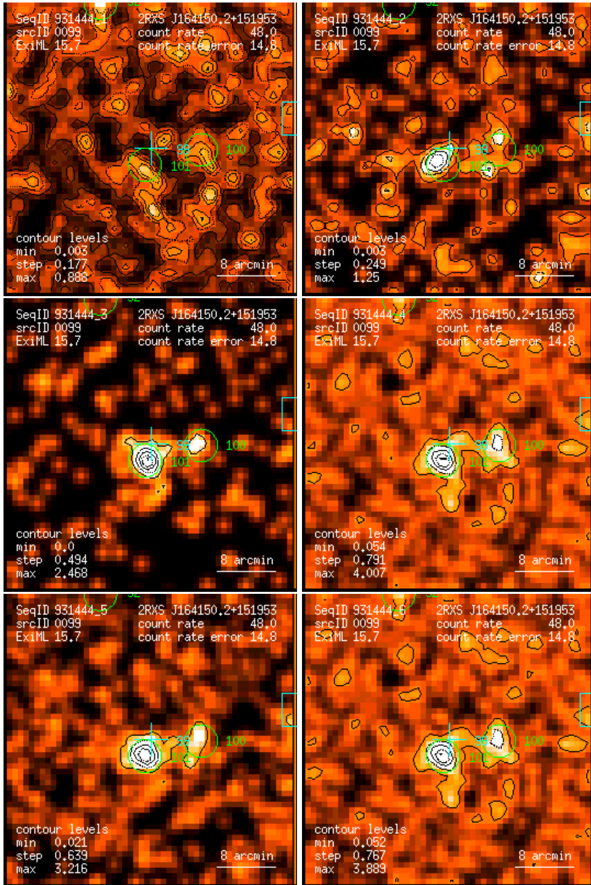
Figure 99: RASS 931444: detection 0099: band rate images, Gaussian filter: (1) PSPC channels 11 – 41, (2) 52 – 90, (3) 91 – 201, (4) 11 – 235, (5) 52 – 201, (6) 11 – 201. Broad band rates in counts/ks. Band rate contour levels in counts/ks/arcmin 2 .
