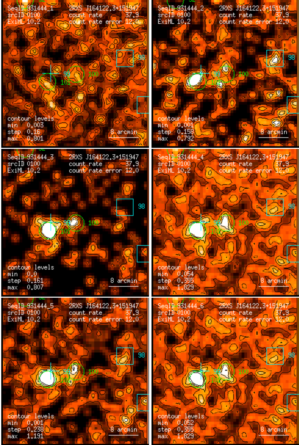
Figure 100: RASS 931444: detection 0100: band rate images, Gaussian filter: (1) PSPC channels 11 – 41, (2) 52 – 90, (3) 91 – 201, (4) 11 – 235, (5) 52 – 201, (6) 11 – 201. Broad band rates in counts/ks. Band rate contour levels in counts/ks/arcmin 2 .
