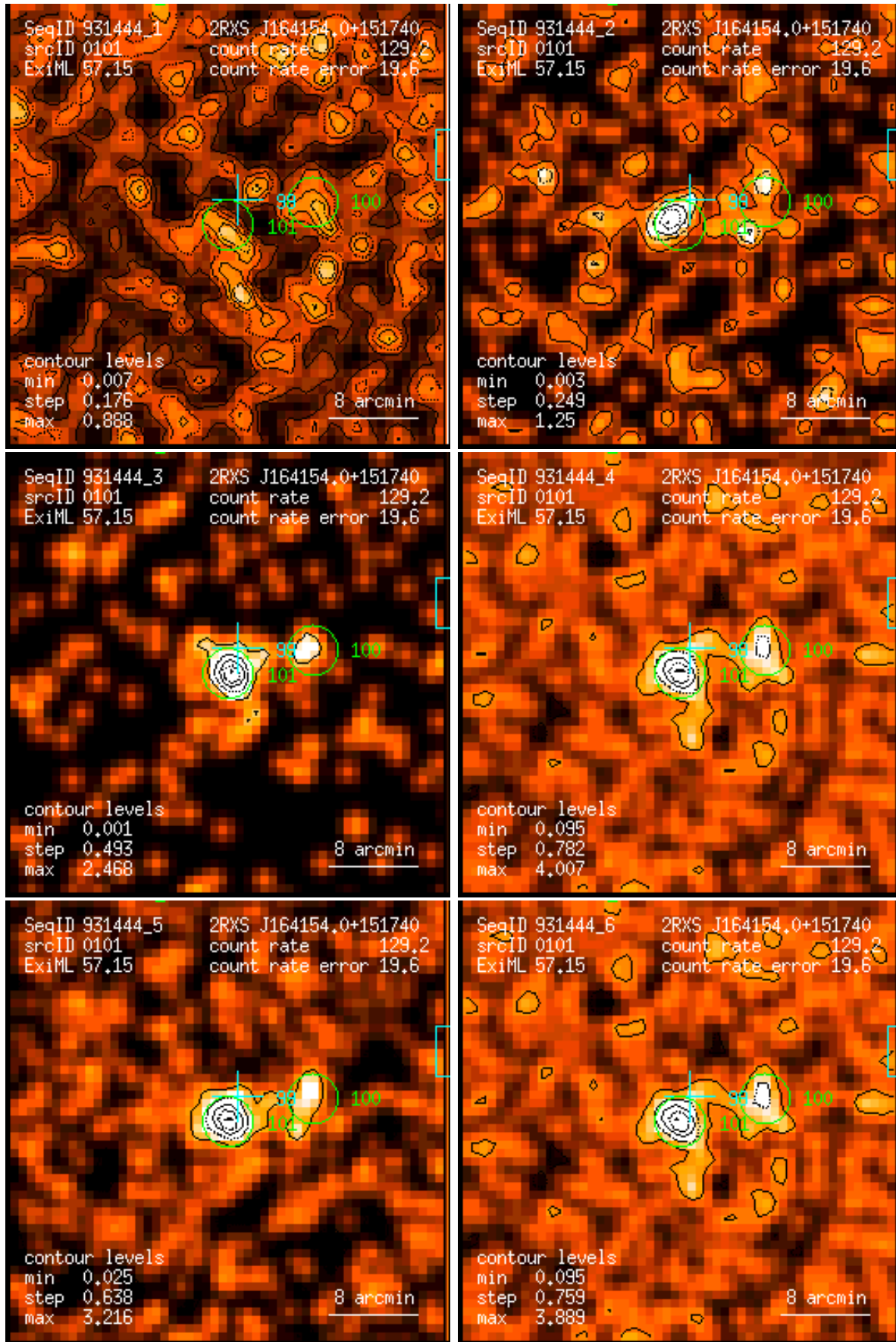
Figure 101: RASS 931444: detection 0101: band rate images, Gaussian filter: (1) PSPC channels 11 – 41, (2) 52 – 90, (3) 91 – 201, (4) 11 – 235, (5) 52 – 201, (6) 11 – 201. Broad band rates in counts/ks. Band rate contour levels in counts/ks/arcmin 2 .
