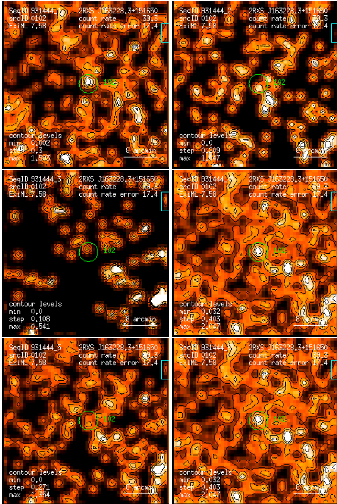
Figure 102: RASS 931444: detection 0102: band rate images, Gaussian filter: (1) PSPC channels 11 – 41, (2) 52 – 90, (3) 91 – 201, (4) 11 – 235, (5) 52 – 201, (6) 11 – 201. Broad band rates in counts/ks. Band rate contour levels in counts/ks/arcmin 2 .
