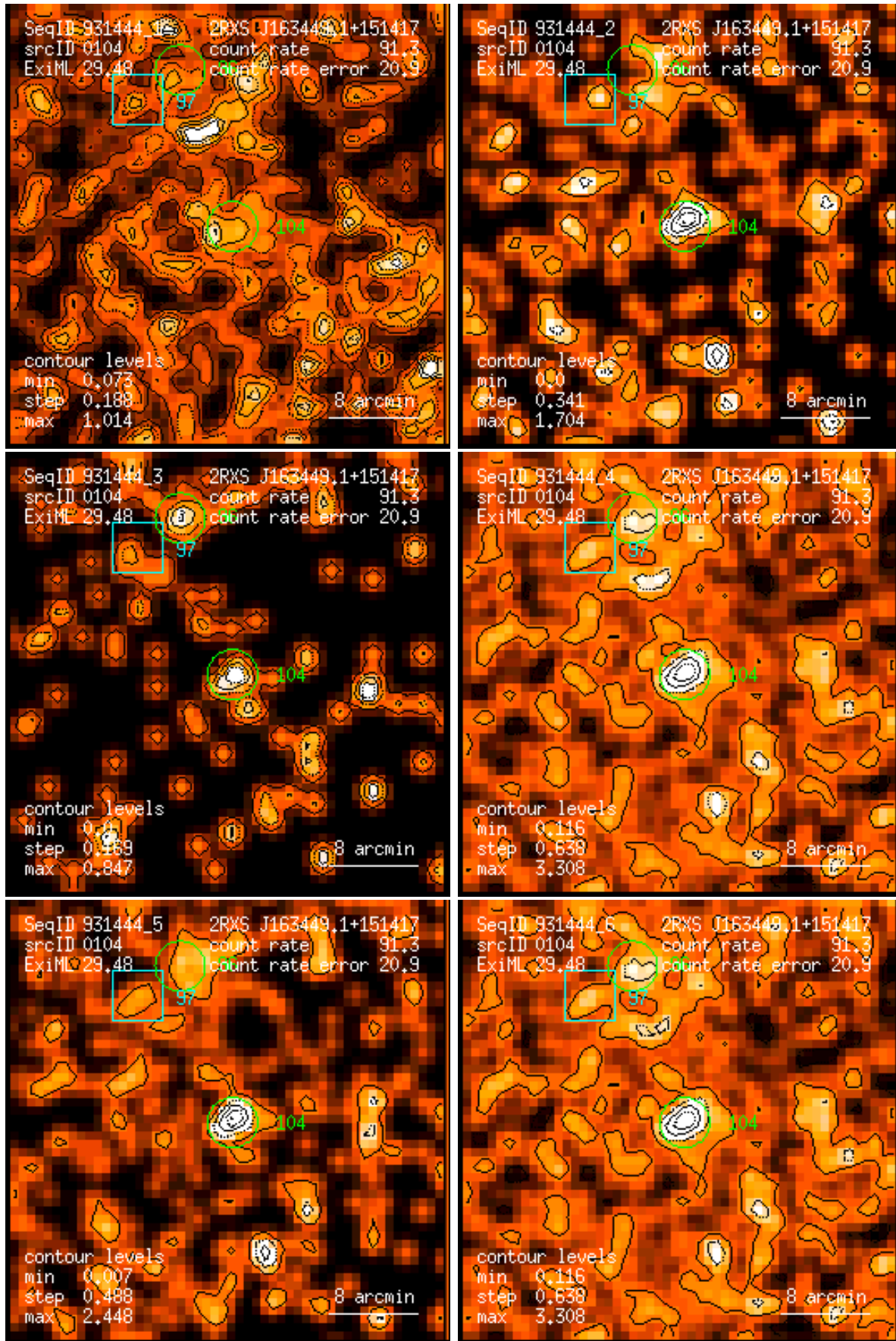
Figure 104: RASS 931444: detection 0104: band rate images, Gaussian filter: (1) PSPC channels 11 – 41, (2) 52 – 90, (3) 91 – 201, (4) 11 – 235, (5) 52 – 201, (6) 11 – 201. Broad band rates in counts/ks. Band rate contour levels in counts/ks/arcmin 2 .
