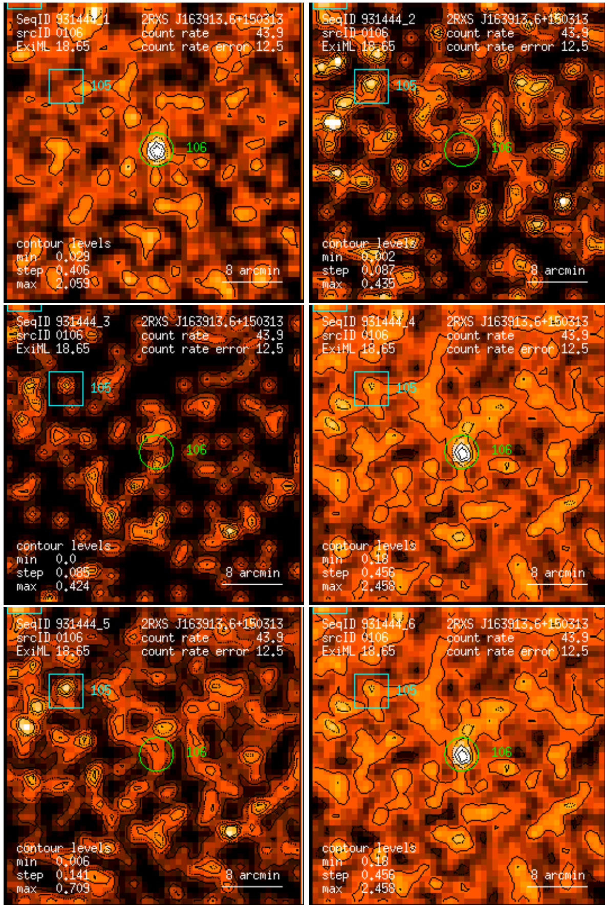
Figure 106: RASS 931444: detection 0106: band rate images, Gaussian filter: (1) PSPC channels 11 – 41, (2) 52 – 90, (3) 91 – 201, (4) 11 – 235, (5) 52 – 201, (6) 11 – 201. Broad band rates in counts/ks. Band rate contour levels in counts/ks/arcmin 2 .
