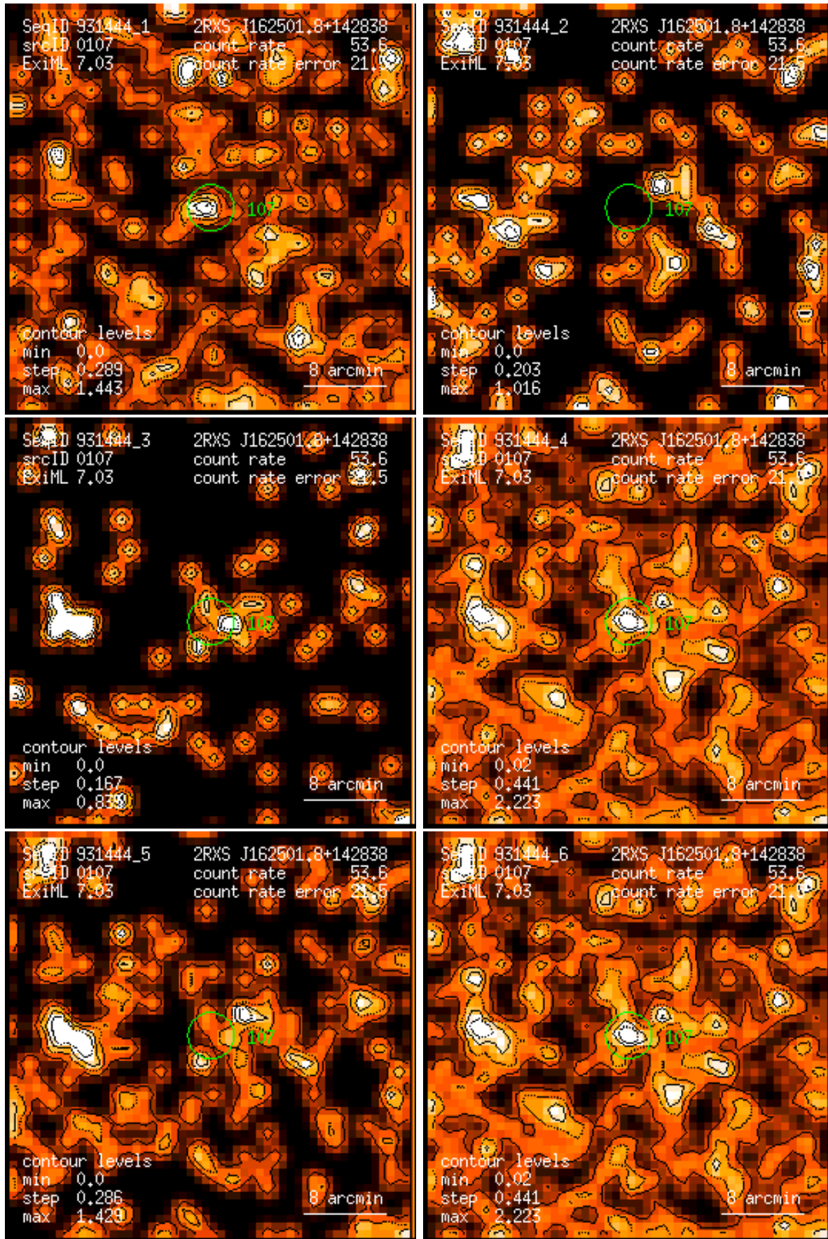
Figure 107: RASS 931444: detection 0107: band rate images, Gaussian filter: (1) PSPC channels 11 – 41, (2) 52 – 90, (3) 91 – 201, (4) 11 – 235, (5) 52 – 201, (6) 11 – 201. Broad band rates in counts/ks. Band rate contour levels in counts/ks/arcmin 2 .
