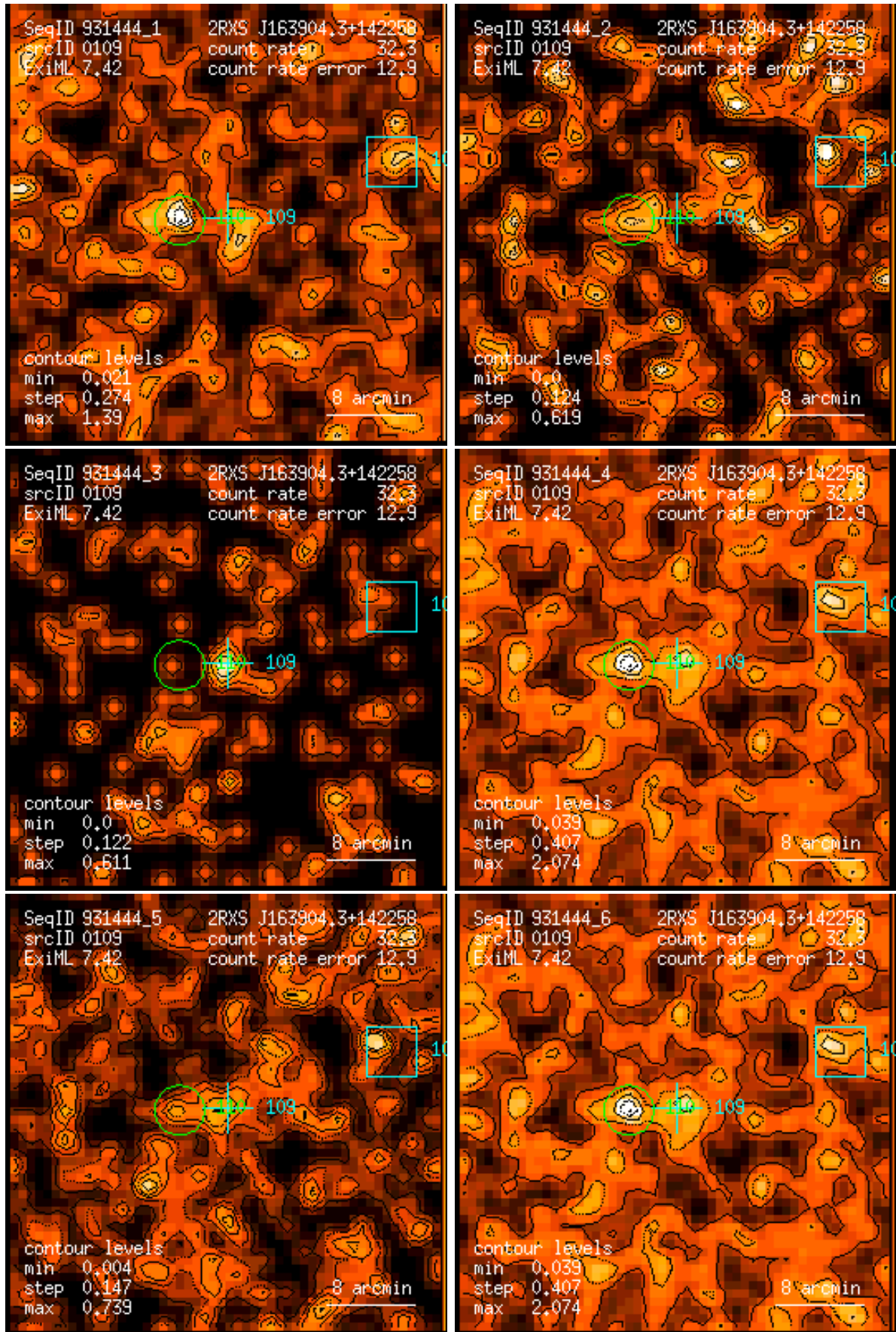
Figure 109: RASS 931444: detection 0109: band rate images, Gaussian filter: (1) PSPC channels 11 – 41, (2) 52 – 90, (3) 91 – 201, (4) 11 – 235, (5) 52 – 201, (6) 11 – 201. Broad band rates in counts/ks. Band rate contour levels in counts/ks/arcmin 2 .
