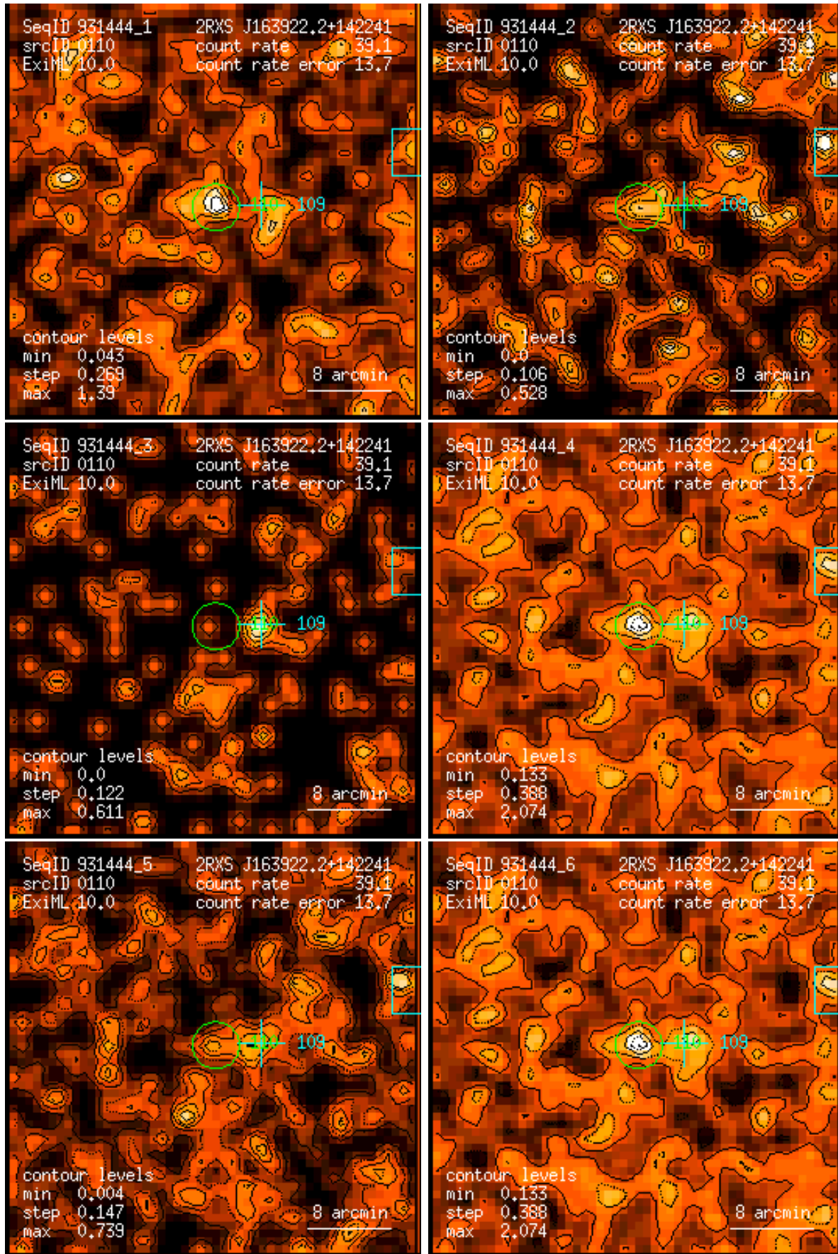
Figure 110: RASS 931444: detection 0110: band rate images, Gaussian filter: (1) PSPC channels 11 – 41, (2) 52 – 90, (3) 91 – 201, (4) 11 – 235, (5) 52 – 201, (6) 11 – 201. Broad band rates in counts/ks. Band rate contour levels in counts/ks/arcmin 2 .
