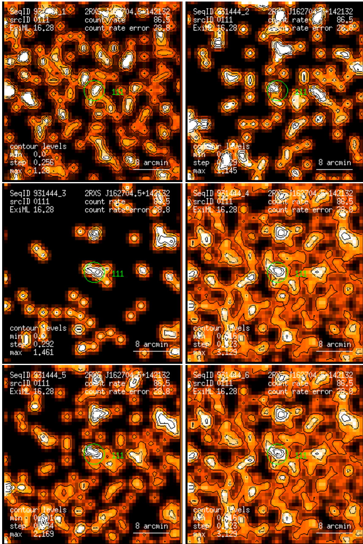
Figure 111: RASS 931444: detection 0111: band rate images, Gaussian filter: (1) PSPC channels 11 – 41, (2) 52 – 90, (3) 91 – 201, (4) 11 – 235, (5) 52 – 201, (6) 11 – 201. Broad band rates in counts/ks. Band rate contour levels in counts/ks/arcmin 2 .
