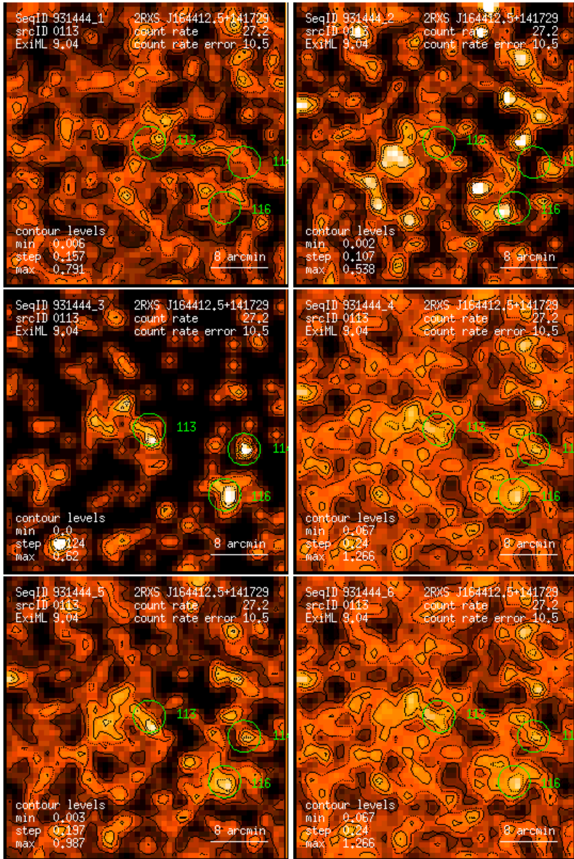
Figure 113: RASS 931444: detection 0113: band rate images, Gaussian filter: (1) PSPC channels 11 – 41, (2) 52 – 90, (3) 91 – 201, (4) 11 – 235, (5) 52 – 201, (6) 11 – 201. Broad band rates in counts/ks. Band rate contour levels in counts/ks/arcmin 2 .
