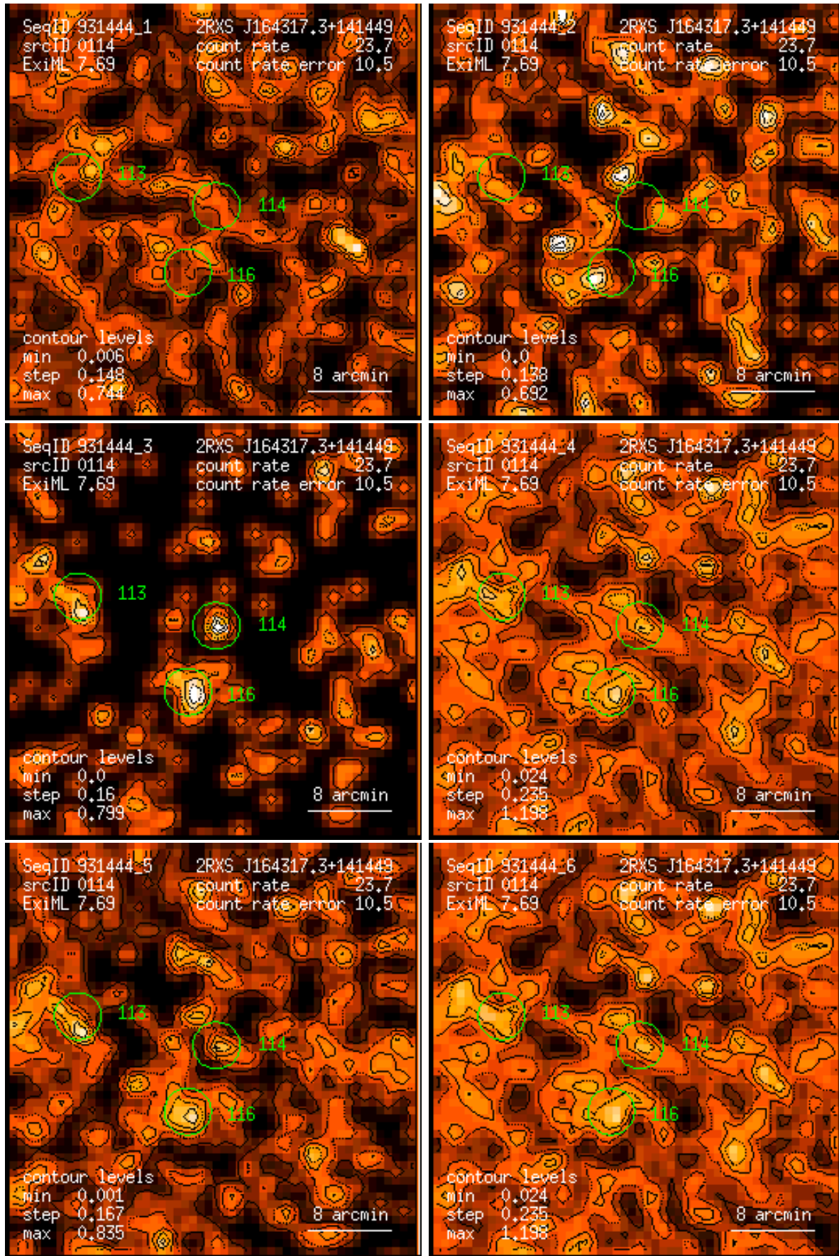
Figure 114: RASS 931444: detection 0114: band rate images, Gaussian filter: (1) PSPC channels 11 – 41, (2) 52 – 90, (3) 91 – 201, (4) 11 – 235, (5) 52 – 201, (6) 11 – 201. Broad band rates in counts/ks. Band rate contour levels in counts/ks/arcmin 2 .
