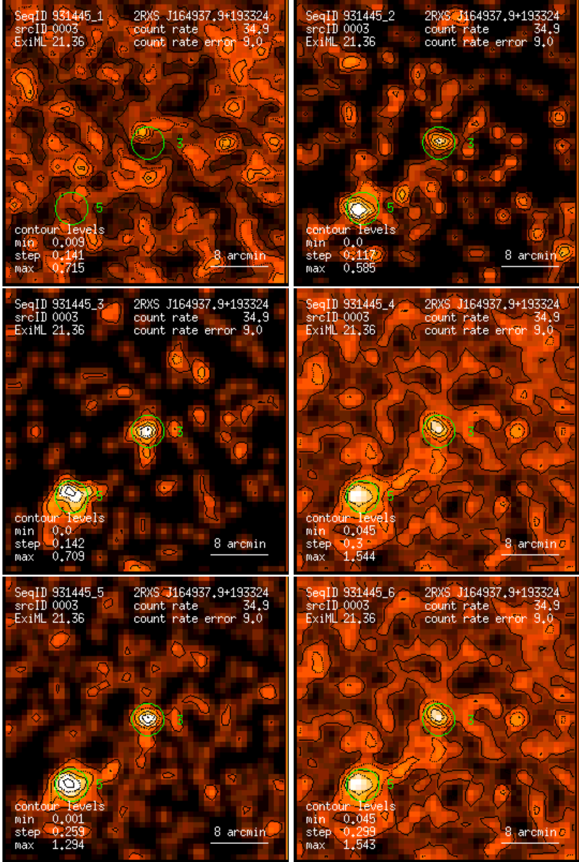
Figure 3: RASS 931445: detection 0003: band rate images, Gaussian filter: (1) PSPC channels 11 – 41, (2) 52 – 90, (3) 91 – 201, (4) 11 – 235, (5) 52 – 201, (6) 11 – 201. Broad band rates in counts/ks. Band rate contour levels in counts/ks/arcmin 2 .
