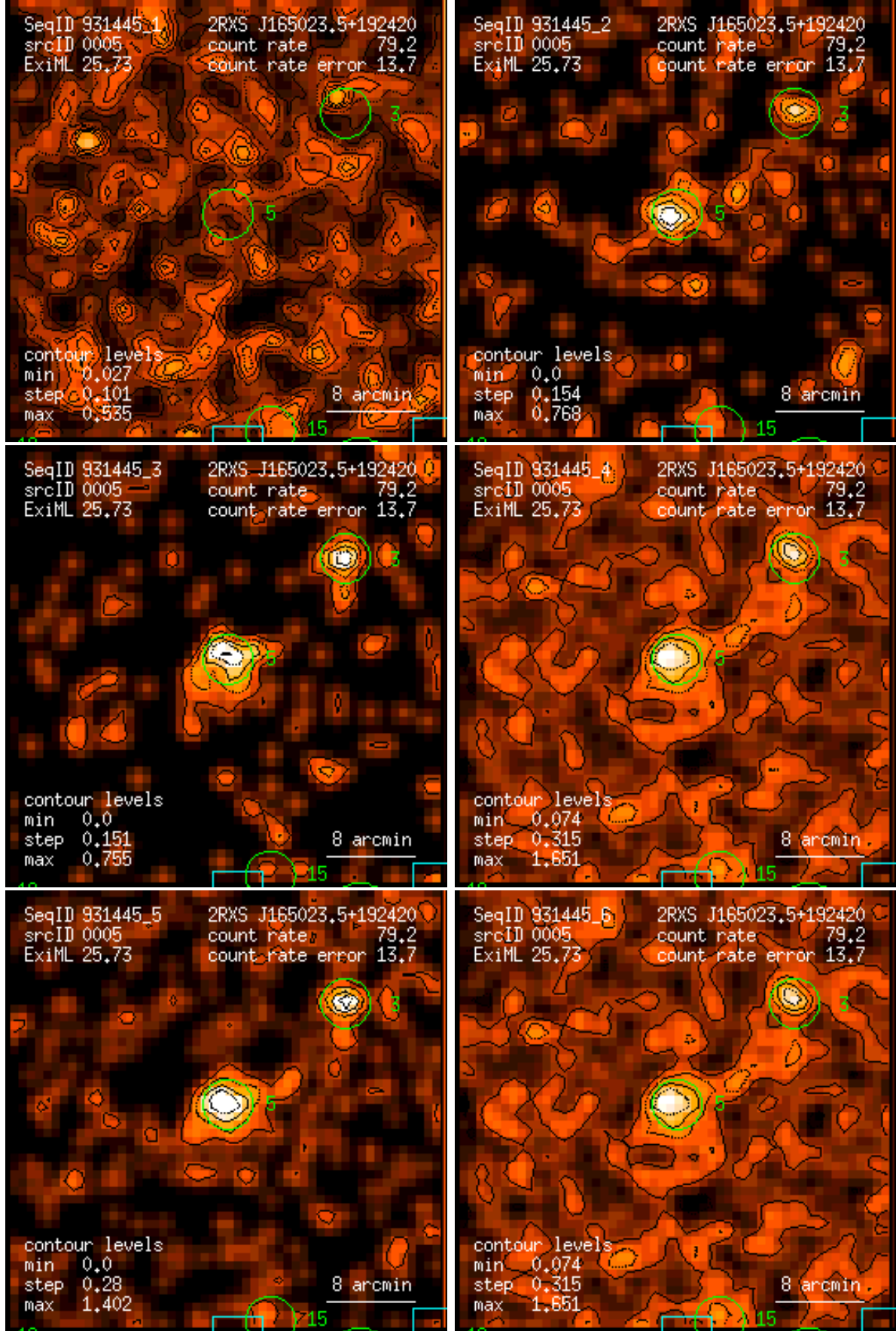
Figure 5: RASS 931445: detection 0005: band rate images, Gaussian filter: (1) PSPC channels 11 – 41, (2) 52 – 90, (3) 91 – 201, (4) 11 – 235, (5) 52 – 201, (6) 11 – 201. Broad band rates in counts/ks. Band rate contour levels in counts/ks/arcmin 2 .
