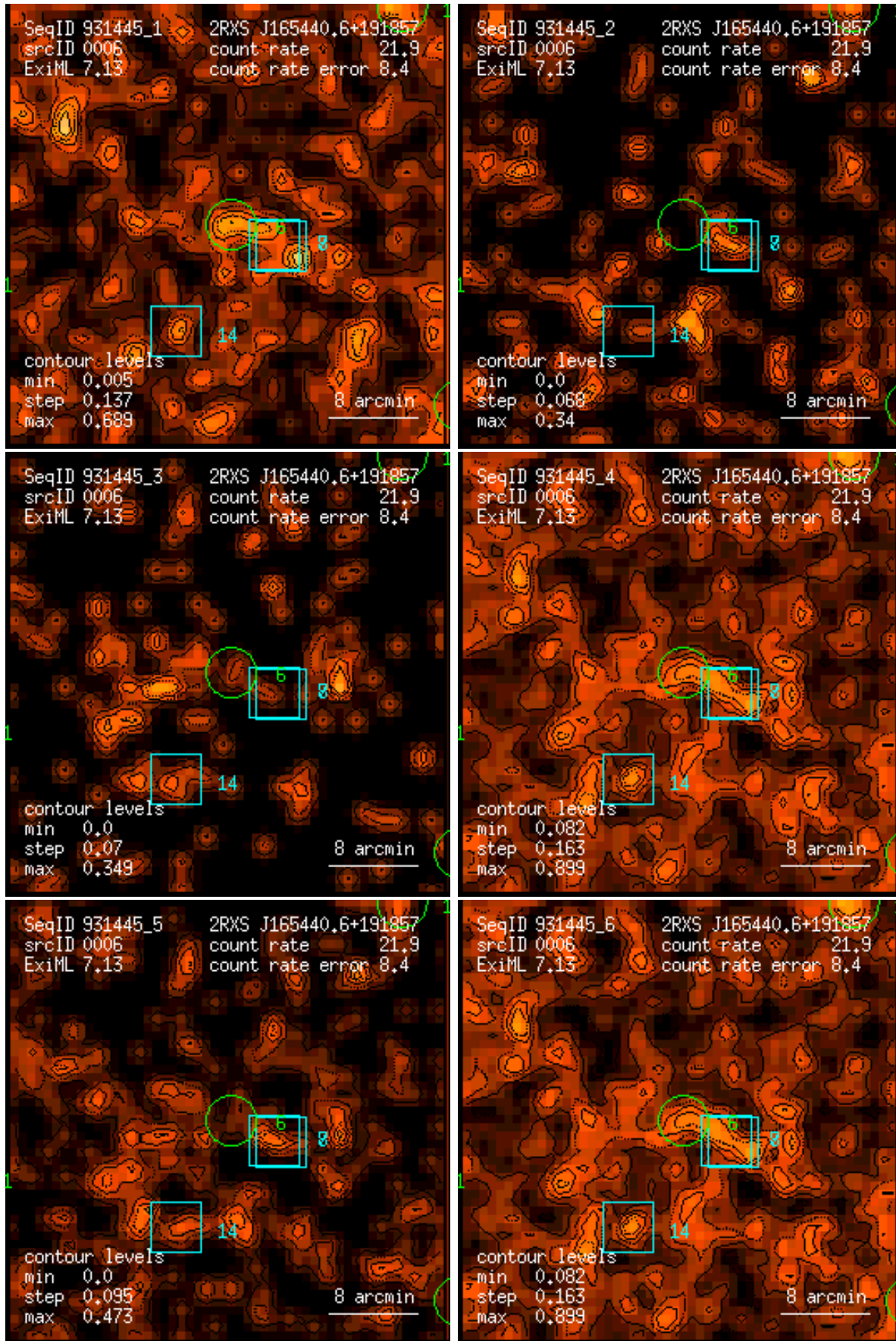
Figure 6: RASS 931445: detection 0006: band rate images, Gaussian filter: (1) PSPC channels 11 – 41, (2) 52 – 90, (3) 91 – 201, (4) 11 – 235, (5) 52 – 201, (6) 11 – 201. Broad band rates in counts/ks. Band rate contour levels in counts/ks/arcmin 2 .
